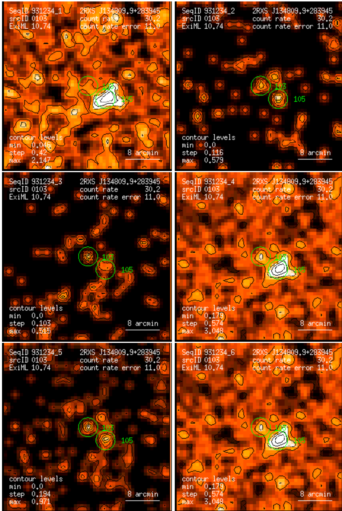
Figure 103: RASS 931234: detection 0103: band rate images, Gaussian filter: (1) PSPC channels 11 – 41, (2) 52 – 90, (3) 91 – 201, (4) 11 – 235, (5) 52 – 201, (6) 11 – 201. Broad band rates in counts/ks. Band rate contour levels in counts/ks/arcmin 2 .
