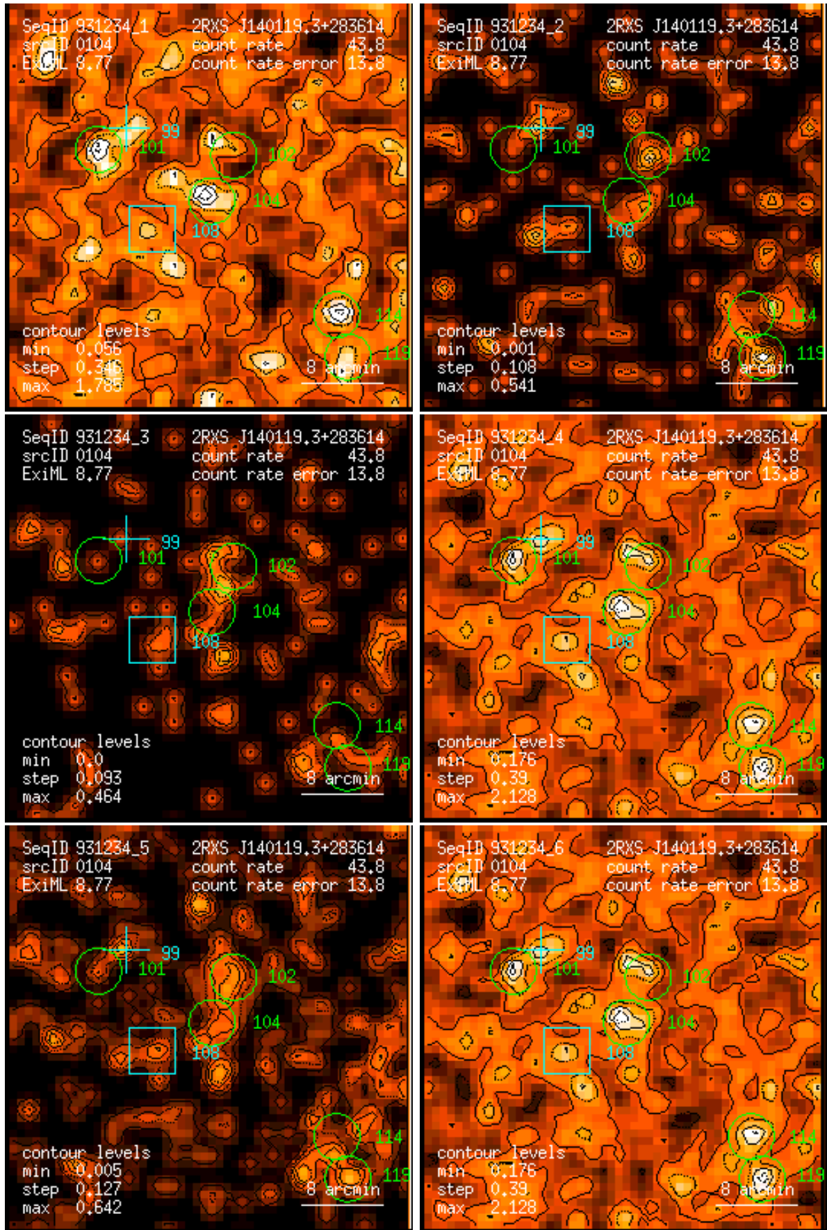
Figure 104: RASS 931234: detection 0104: band rate images, Gaussian filter: (1) PSPC channels 11 – 41, (2) 52 – 90, (3) 91 – 201, (4) 11 – 235, (5) 52 – 201, (6) 11 – 201. Broad band rates in counts/ks. Band rate contour levels in counts/ks/arcmin 2 .
