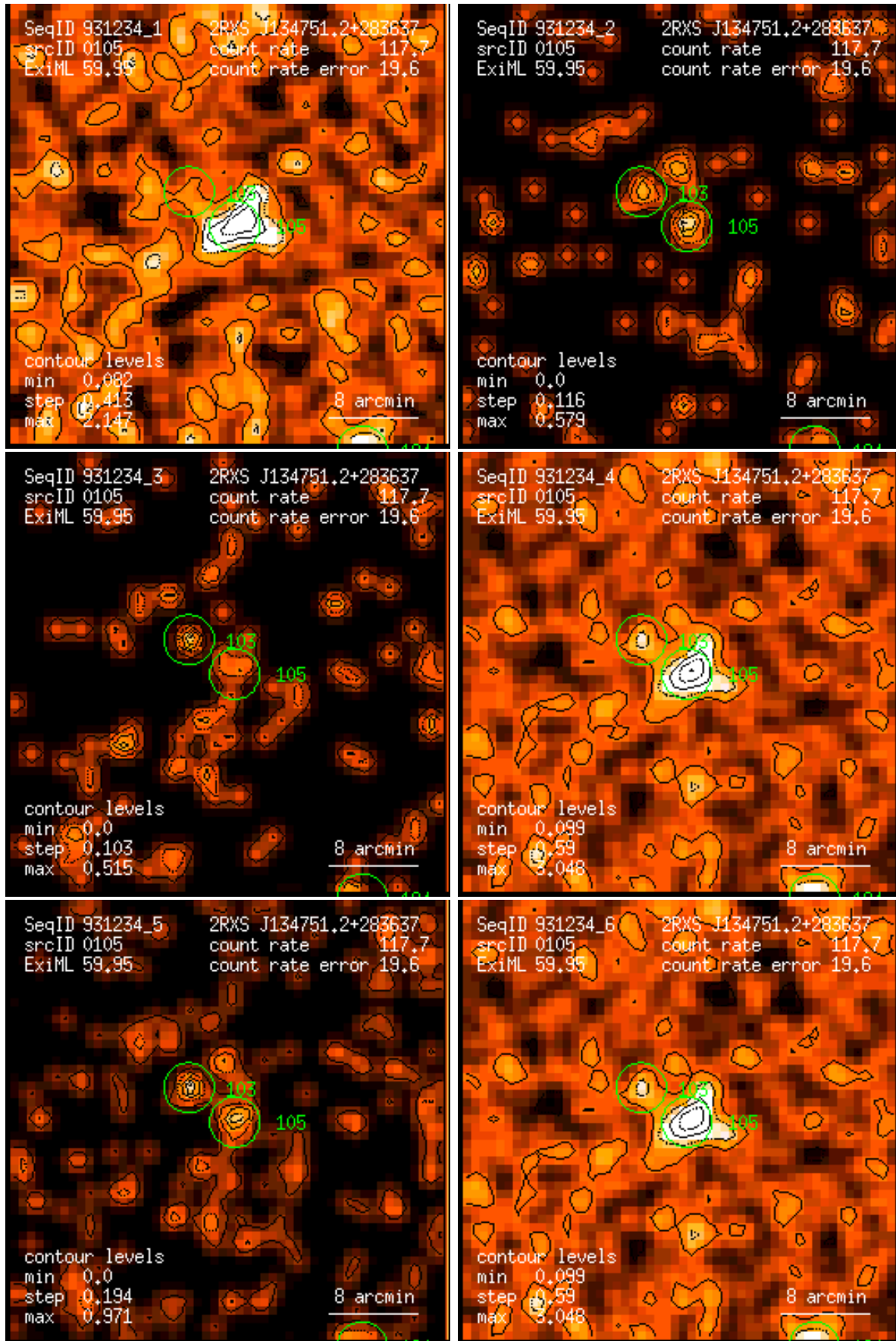
Figure 105: RASS 931234: detection 0105: band rate images, Gaussian filter: (1) PSPC channels 11 – 41, (2) 52 – 90, (3) 91 – 201, (4) 11 – 235, (5) 52 – 201, (6) 11 – 201. Broad band rates in counts/ks. Band rate contour levels in counts/ks/arcmin 2 .
