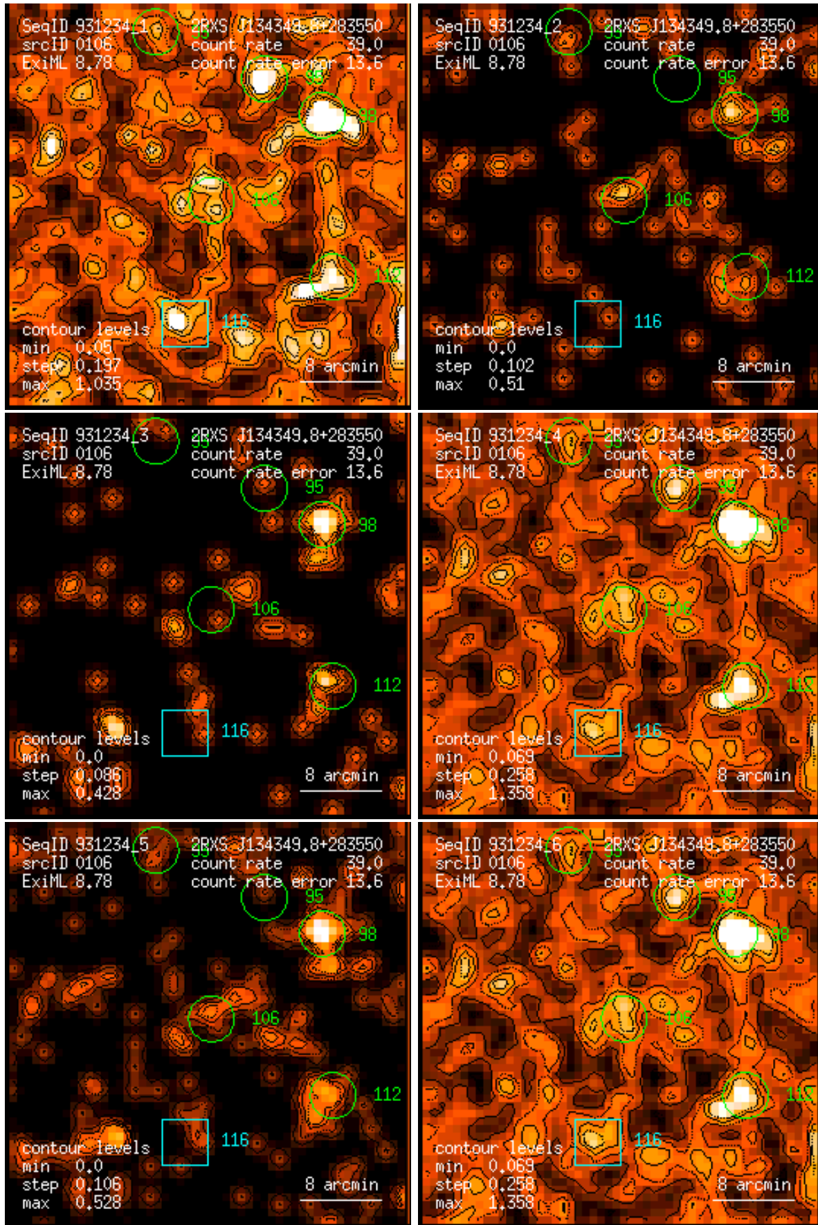
Figure 106: RASS 931234: detection 0106: band rate images, Gaussian filter: (1) PSPC channels 11 – 41, (2) 52 – 90, (3) 91 – 201, (4) 11 – 235, (5) 52 – 201, (6) 11 – 201. Broad band rates in counts/ks. Band rate contour levels in counts/ks/arcmin 2 .
