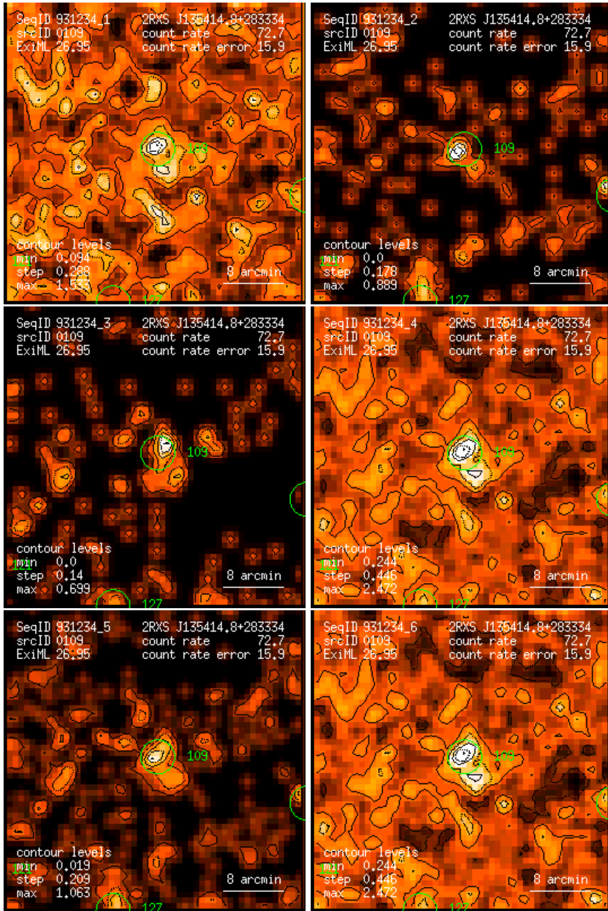
Figure 109: RASS 931234: detection 0109: band rate images, Gaussian filter: (1) PSPC channels 11 – 41, (2) 52 – 90, (3) 91 – 201, (4) 11 – 235, (5) 52 – 201, (6) 11 – 201. Broad band rates in counts/ks. Band rate contour levels in counts/ks/arcmin 2 .
