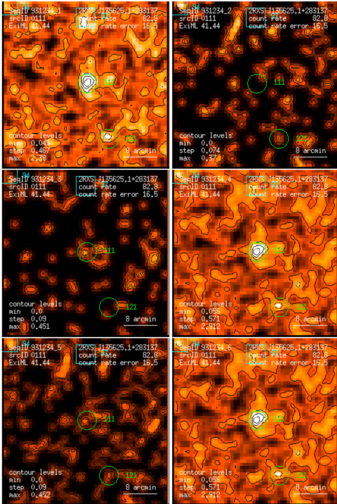
Figure 111: RASS 931234: detection 0111: band rate images, Gaussian filter: (1) PSPC channels 11 – 41, (2) 52 – 90, (3) 91 – 201, (4) 11 – 235, (5) 52 – 201, (6) 11 – 201. Broad band rates in counts/ks. Band rate contour levels in counts/ks/arcmin 2 .
