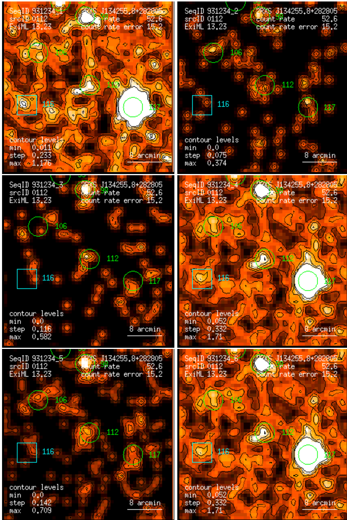
Figure 112: RASS 931234: detection 0112: band rate images, Gaussian filter: (1) PSPC channels 11 – 41, (2) 52 – 90, (3) 91 – 201, (4) 11 – 235, (5) 52 – 201, (6) 11 – 201. Broad band rates in counts/ks. Band rate contour levels in counts/ks/arcmin 2 .
