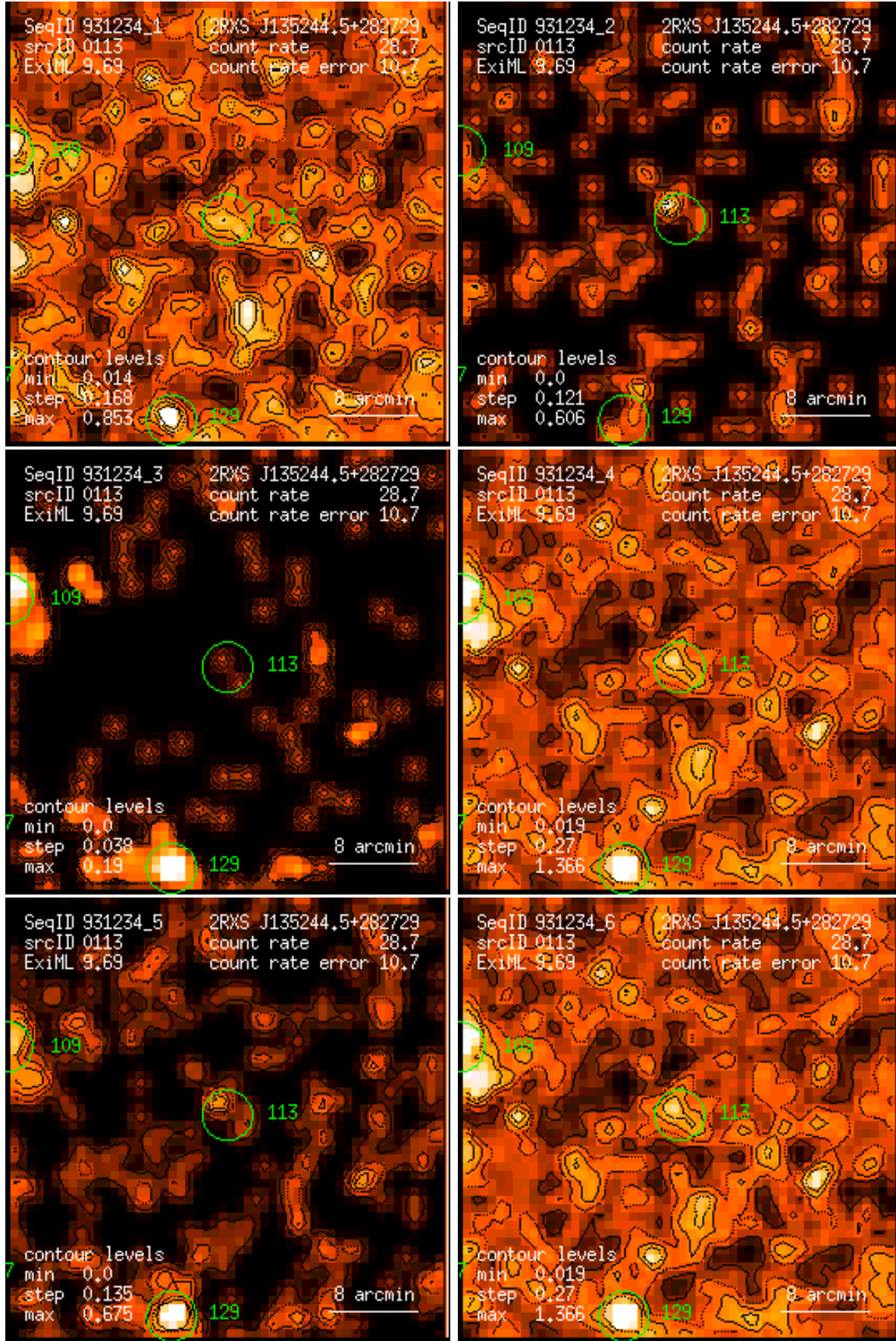
Figure 113: RASS 931234: detection 0113: band rate images, Gaussian filter: (1) PSPC channels 11 – 41, (2) 52 – 90, (3) 91 – 201, (4) 11 – 235, (5) 52 – 201, (6) 11 – 201. Broad band rates in counts/ks. Band rate contour levels in counts/ks/arcmin 2 .
