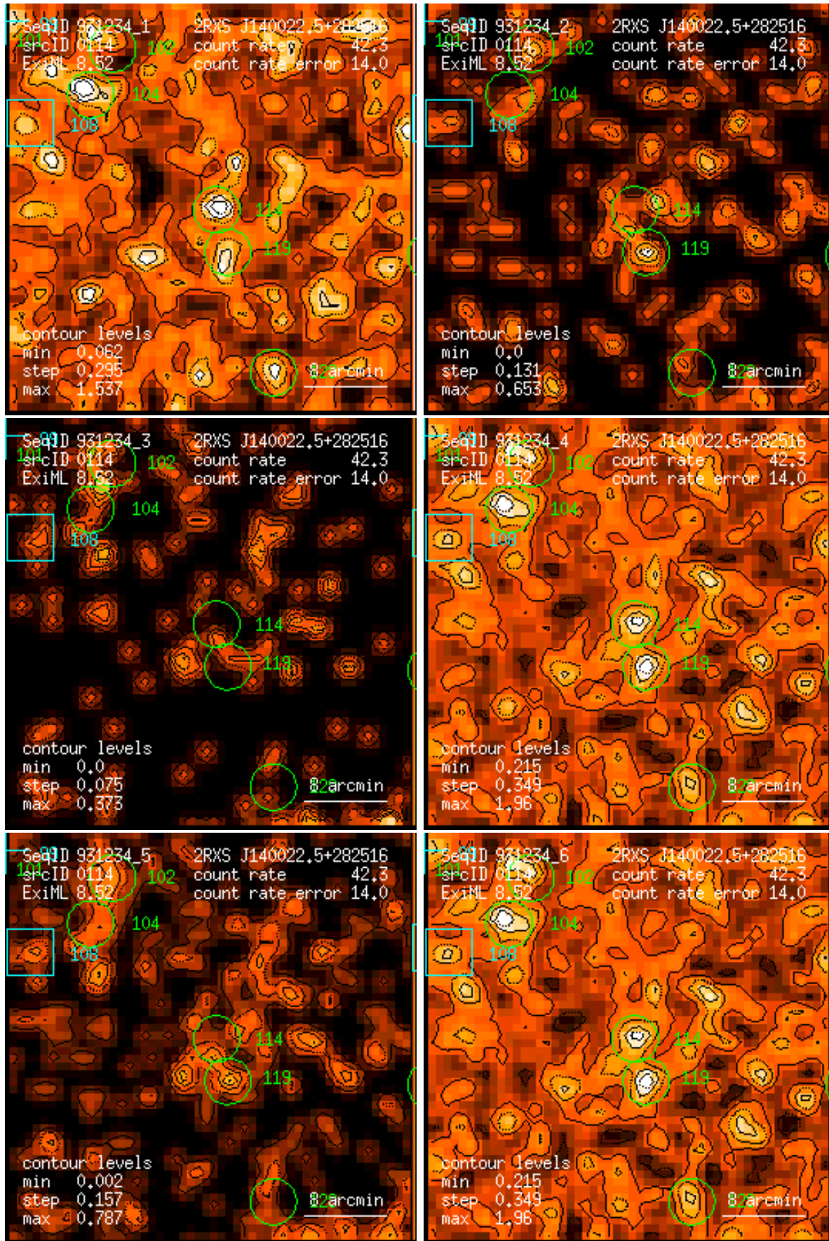
Figure 114: RASS 931234: detection 0114: band rate images, Gaussian filter: (1) PSPC channels 11 – 41, (2) 52 – 90, (3) 91 – 201, (4) 11 – 235, (5) 52 – 201, (6) 11 – 201. Broad band rates in counts/ks. Band rate contour levels in counts/ks/arcmin 2 .
