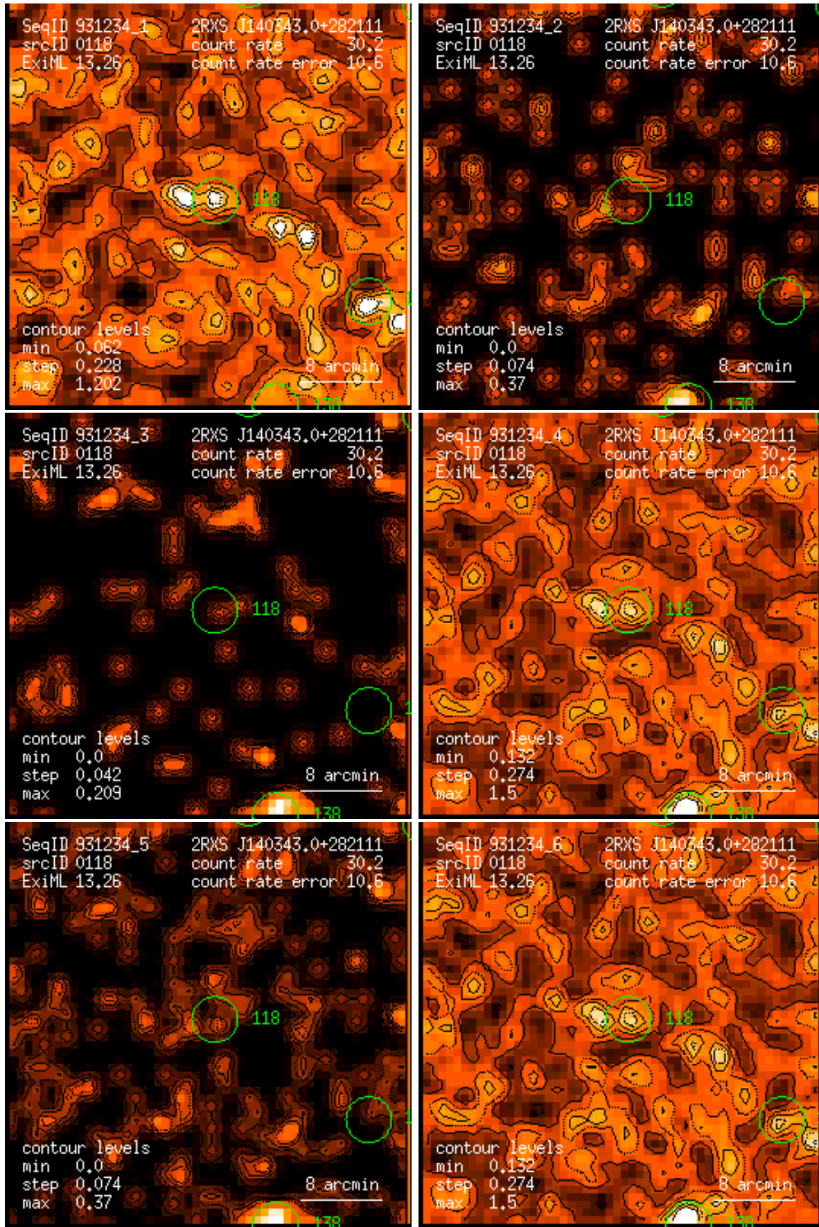
Figure 118: RASS 931234: detection 0118: band rate images, Gaussian filter: (1) PSPC channels 11 – 41, (2) 52 – 90, (3) 91 – 201, (4) 11 – 235, (5) 52 – 201, (6) 11 – 201. Broad band rates in counts/ks. Band rate contour levels in counts/ks/arcmin 2 .
