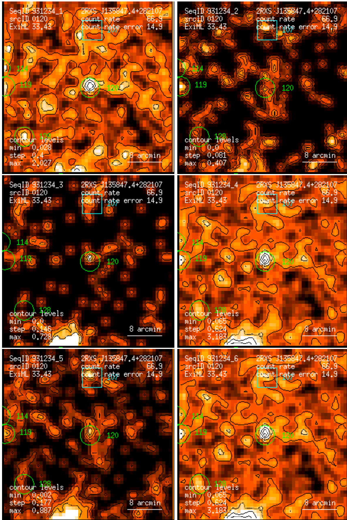
Figure 120: RASS 931234: detection 0120: band rate images, Gaussian filter: (1) PSPC channels 11 – 41, (2) 52 – 90, (3) 91 – 201, (4) 11 – 235, (5) 52 – 201, (6) 11 – 201. Broad band rates in counts/ks. Band rate contour levels in counts/ks/arcmin 2 .
