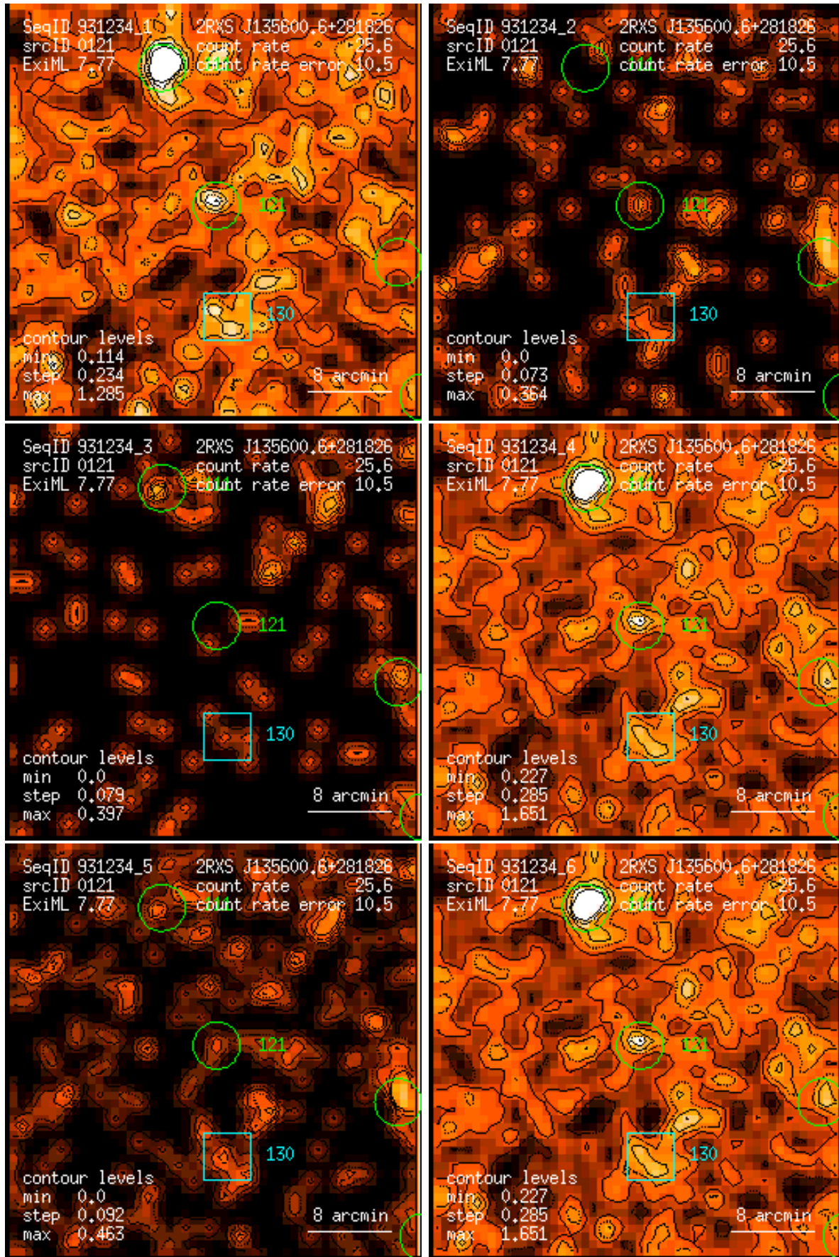
Figure 121: RASS 931234: detection 0121: band rate images, Gaussian filter: (1) PSPC channels 11 – 41, (2) 52 – 90, (3) 91 – 201, (4) 11 – 235, (5) 52 – 201, (6) 11 – 201. Broad band rates in counts/ks. Band rate contour levels in counts/ks/arcmin 2 .
