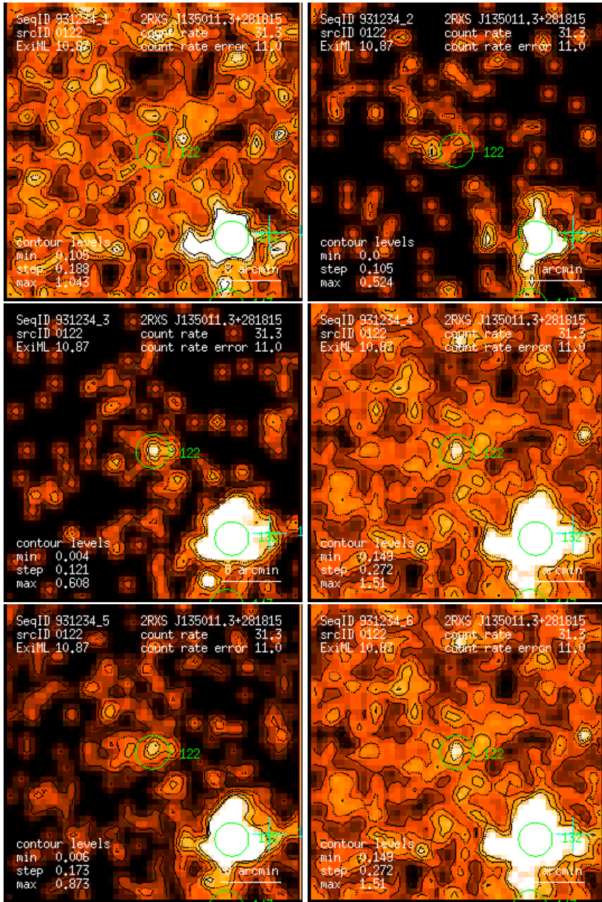
Figure 122: RASS 931234: detection 0122: band rate images, Gaussian filter: (1) PSPC channels 11 – 41, (2) 52 – 90, (3) 91 – 201, (4) 11 – 235, (5) 52 – 201, (6) 11 – 201. Broad band rates in counts/ks. Band rate contour levels in counts/ks/arcmin 2 .
