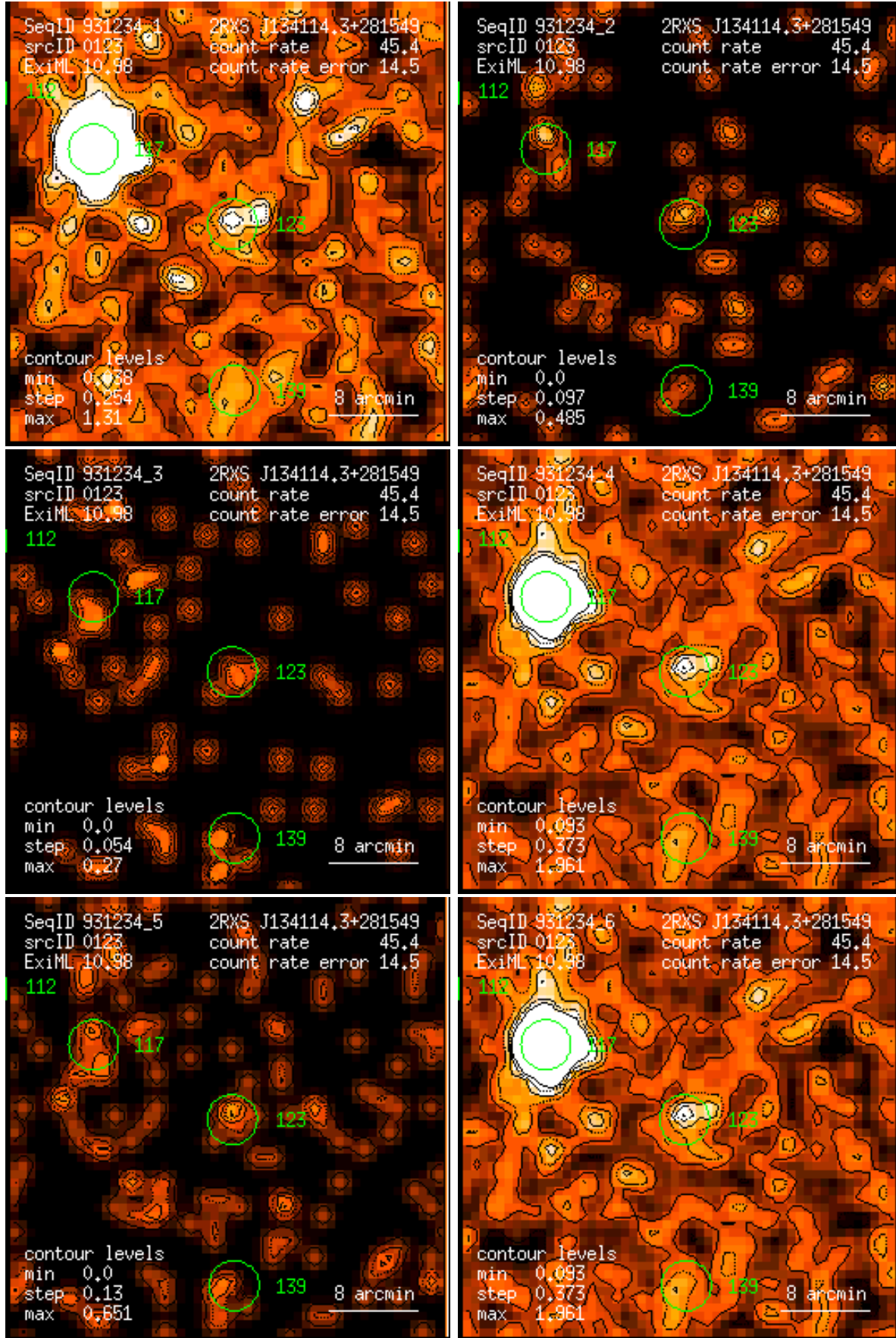
Figure 123: RASS 931234: detection 0123: band rate images, Gaussian filter: (1) PSPC channels 11 – 41, (2) 52 – 90, (3) 91 – 201, (4) 11 – 235, (5) 52 – 201, (6) 11 – 201. Broad band rates in counts/ks. Band rate contour levels in counts/ks/arcmin 2 .
