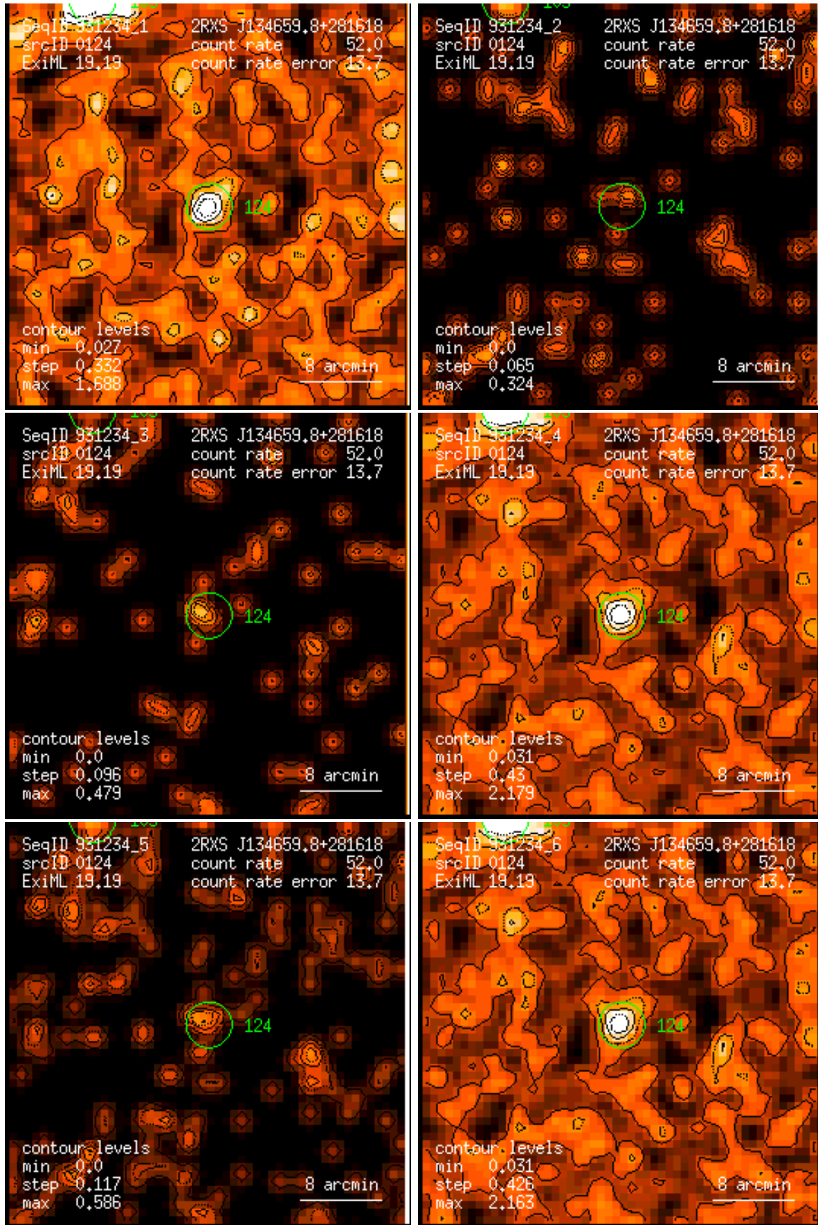
Figure 124: RASS 931234: detection 0124: band rate images, Gaussian filter: (1) PSPC channels 11 – 41, (2) 52 – 90, (3) 91 – 201, (4) 11 – 235, (5) 52 – 201, (6) 11 – 201. Broad band rates in counts/ks. Band rate contour levels in counts/ks/arcmin 2 .
