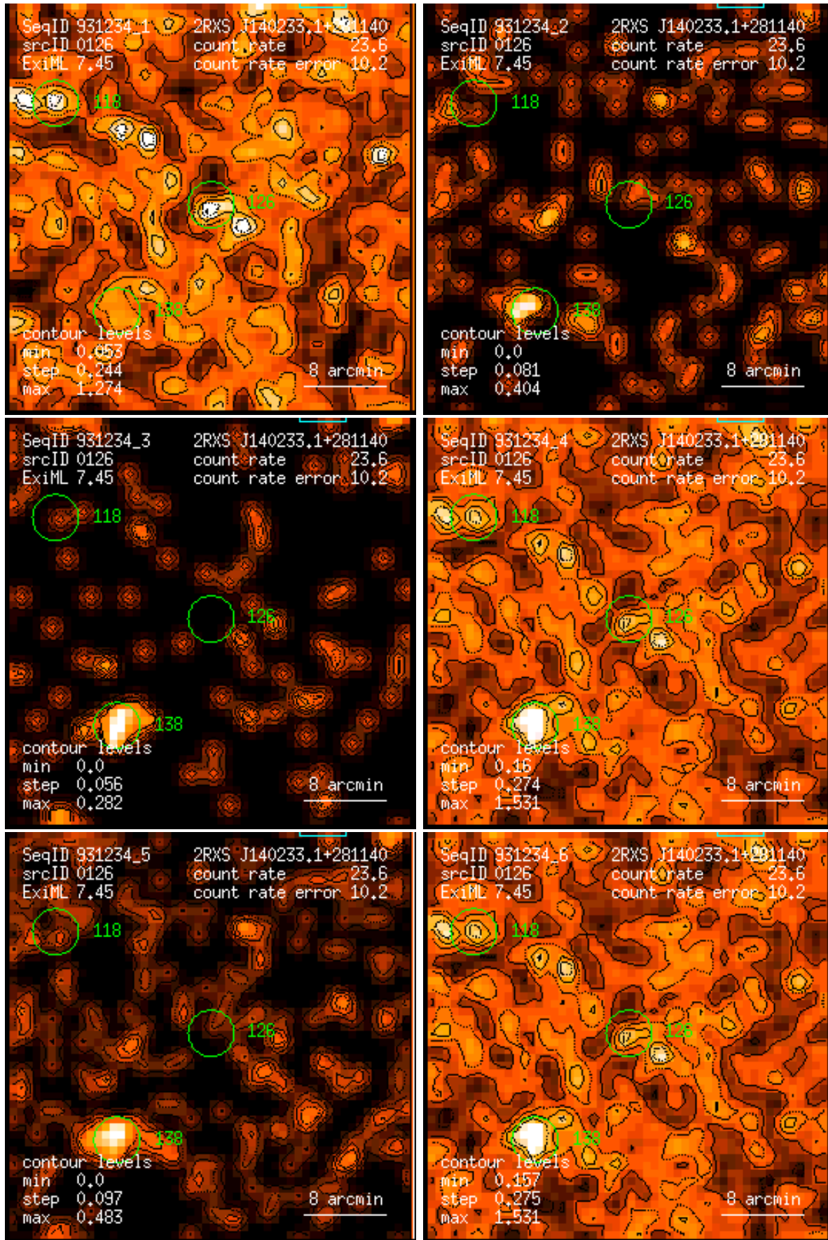
Figure 126: RASS 931234: detection 0126: band rate images, Gaussian filter: (1) PSPC channels 11 – 41, (2) 52 – 90, (3) 91 – 201, (4) 11 – 235, (5) 52 – 201, (6) 11 – 201. Broad band rates in counts/ks. Band rate contour levels in counts/ks/arcmin 2 .
