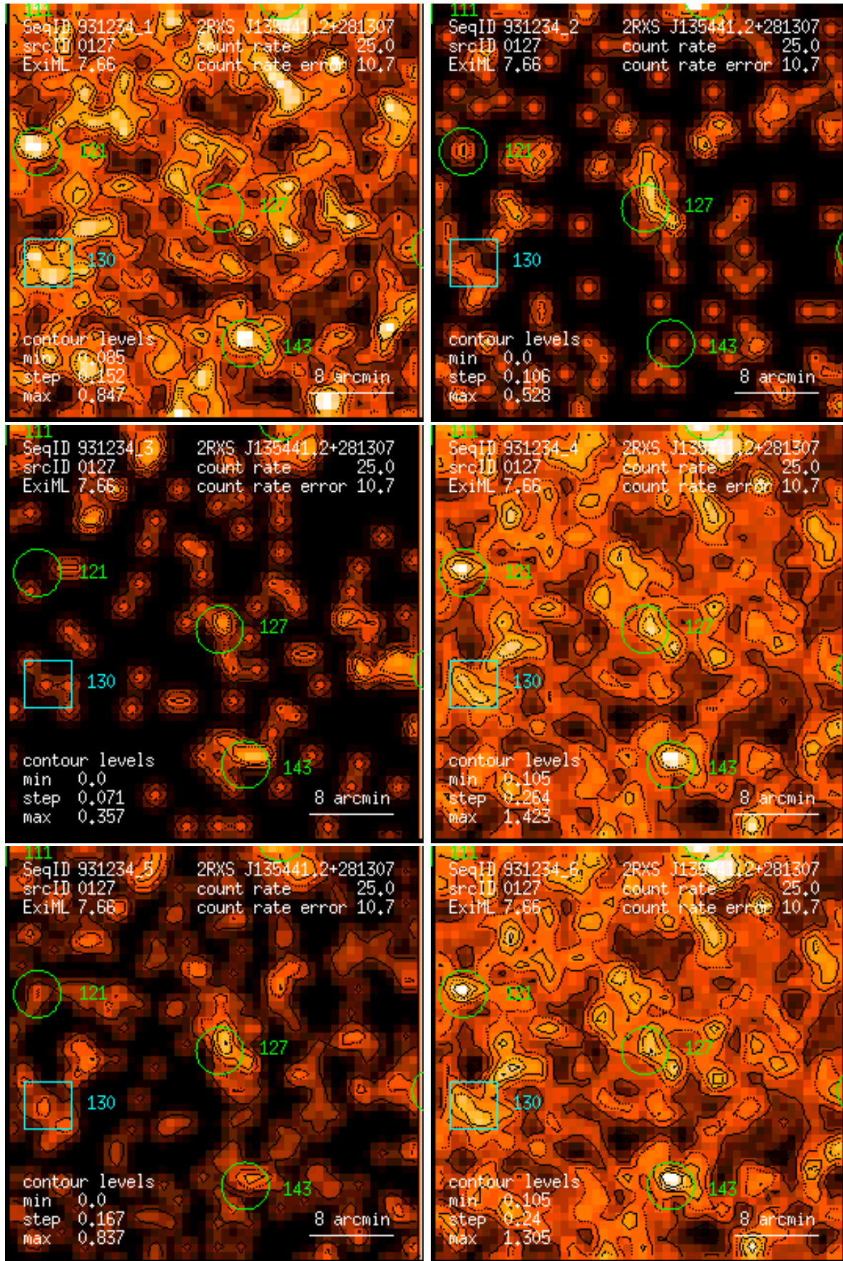
Figure 127: RASS 931234: detection 0127: band rate images, Gaussian filter: (1) PSPC channels 11 – 41, (2) 52 – 90, (3) 91 – 201, (4) 11 – 235, (5) 52 – 201, (6) 11 – 201. Broad band rates in counts/ks. Band rate contour levels in counts/ks/arcmin 2 .
