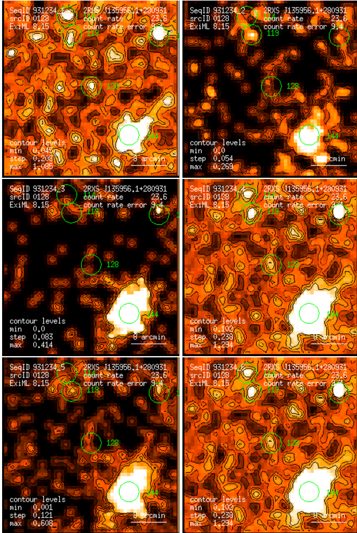
Figure 128: RASS 931234: detection 0128: band rate images, Gaussian filter: (1) PSPC channels 11 – 41, (2) 52 – 90, (3) 91 – 201, (4) 11 – 235, (5) 52 – 201, (6) 11 – 201. Broad band rates in counts/ks. Band rate contour levels in counts/ks/arcmin 2 .
