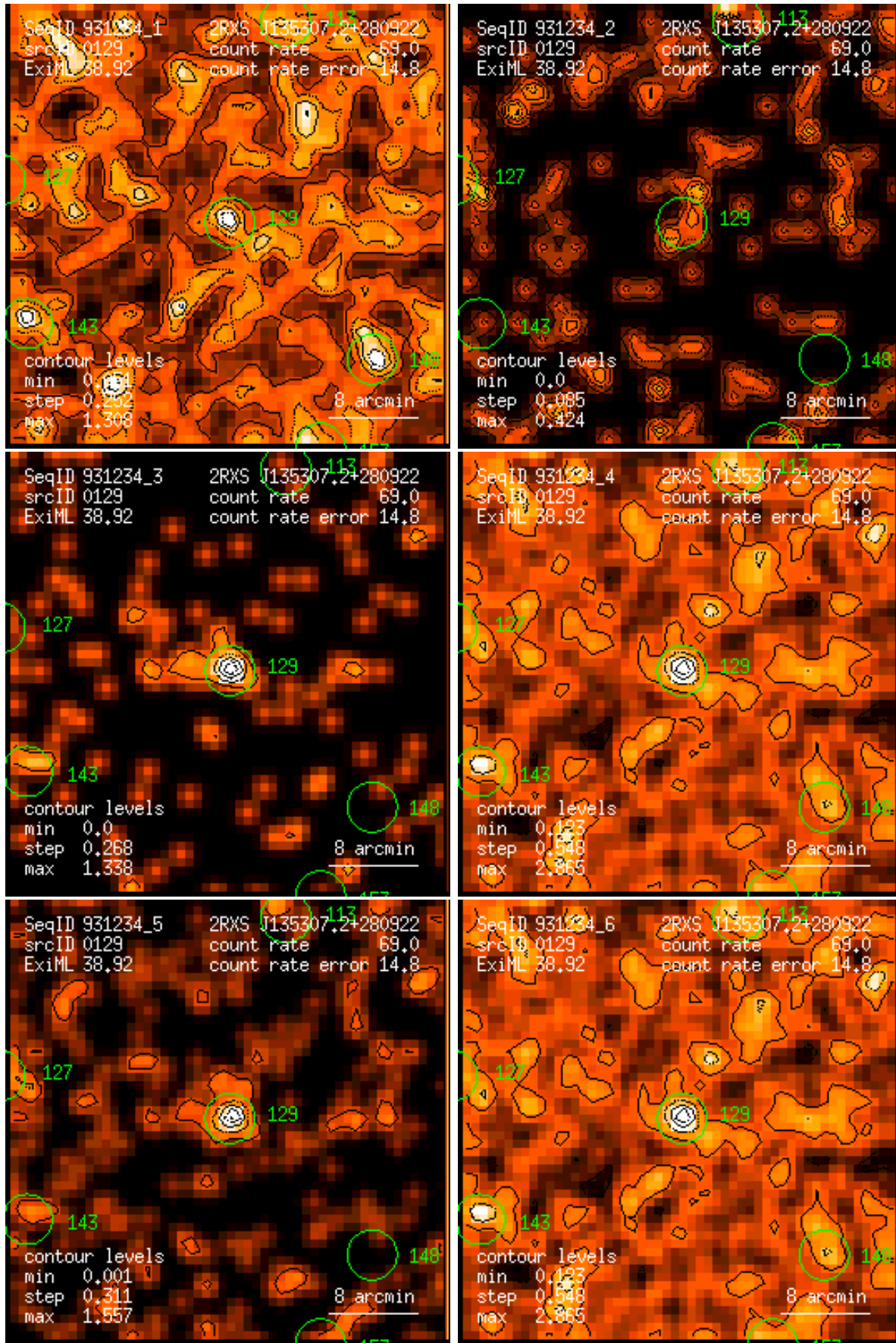
Figure 129: RASS 931234: detection 0129: band rate images, Gaussian filter: (1) PSPC channels 11 – 41, (2) 52 – 90, (3) 91 – 201, (4) 11 – 235, (5) 52 – 201, (6) 11 – 201. Broad band rates in counts/ks. Band rate contour levels in counts/ks/arcmin 2 .
