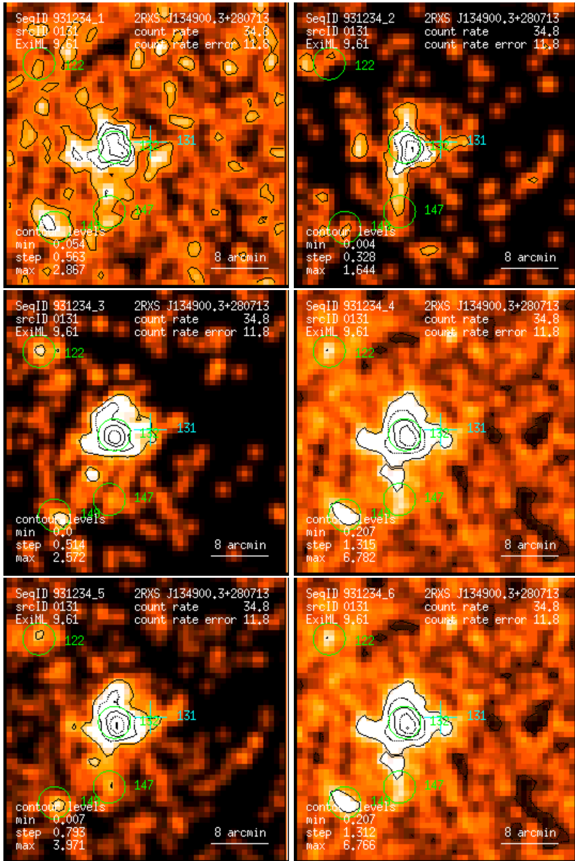
Figure 131: RASS 931234: detection 0131: band rate images, Gaussian filter: (1) PSPC channels 11 – 41, (2) 52 – 90, (3) 91 – 201, (4) 11 – 235, (5) 52 – 201, (6) 11 – 201. Broad band rates in counts/ks. Band rate contour levels in counts/ks/arcmin 2 .
