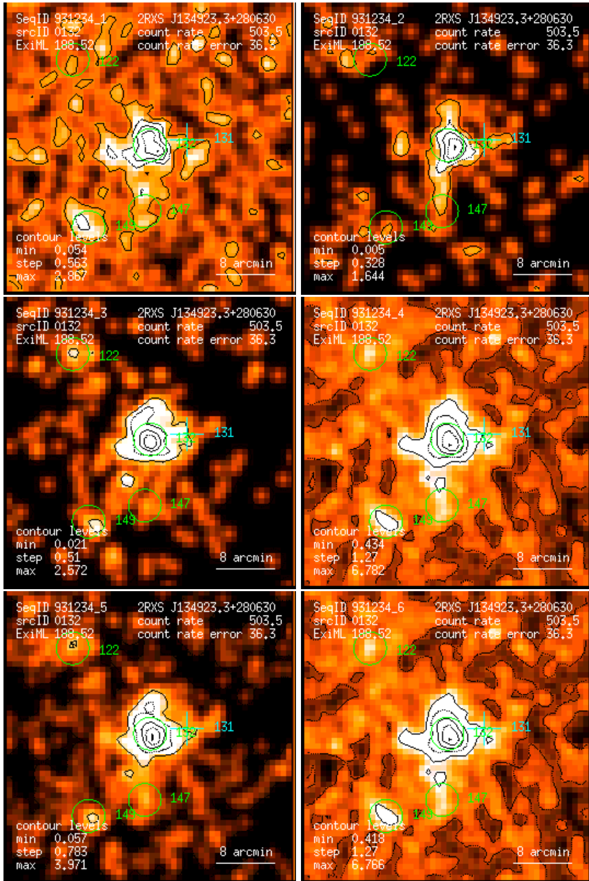
Figure 132: RASS 931234: detection 0132: band rate images, Gaussian filter: (1) PSPC channels 11 – 41, (2) 52 – 90, (3) 91 – 201, (4) 11 – 235, (5) 52 – 201, (6) 11 – 201. Broad band rates in counts/ks. Band rate contour levels in counts/ks/arcmin 2 .
