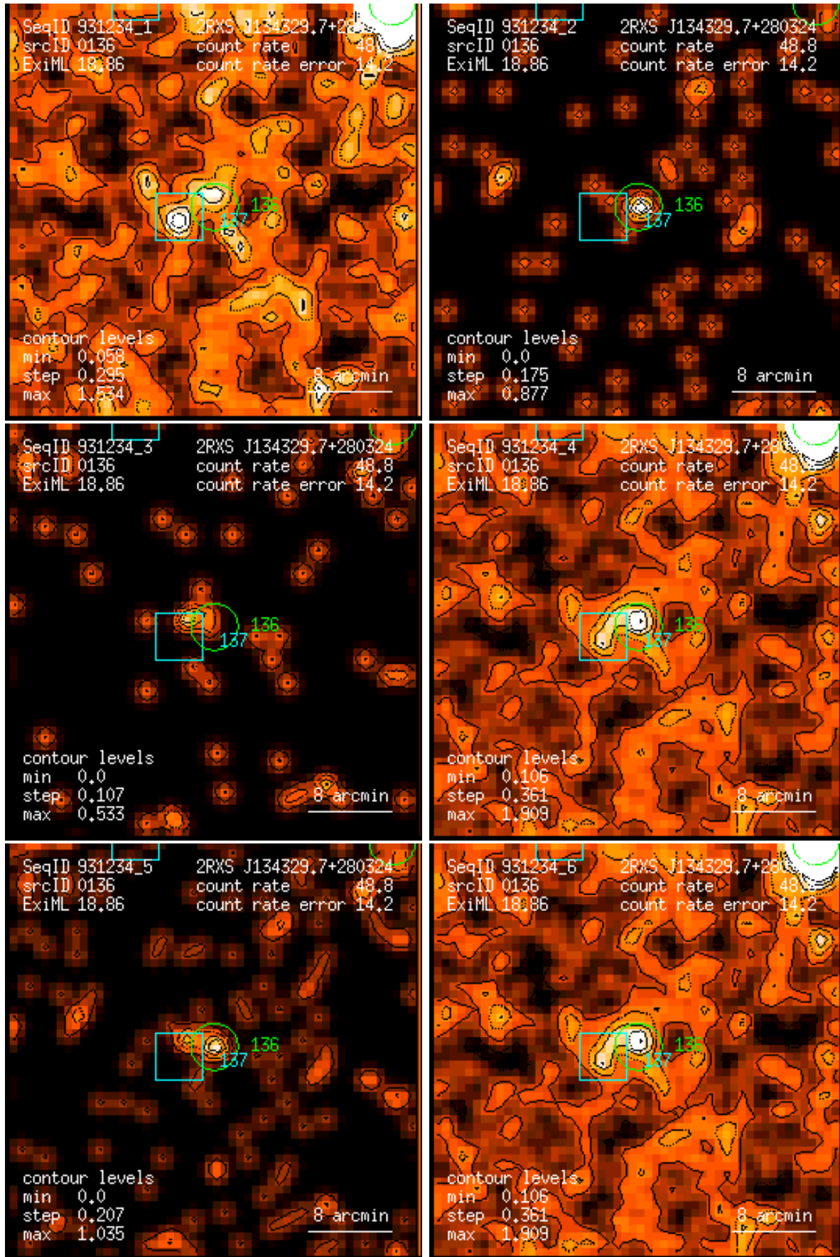
Figure 136: RASS 931234: detection 0136: band rate images, Gaussian filter: (1) PSPC channels 11 – 41, (2) 52 – 90, (3) 91 – 201, (4) 11 – 235, (5) 52 – 201, (6) 11 – 201. Broad band rates in counts/ks. Band rate contour levels in counts/ks/arcmin 2 .
