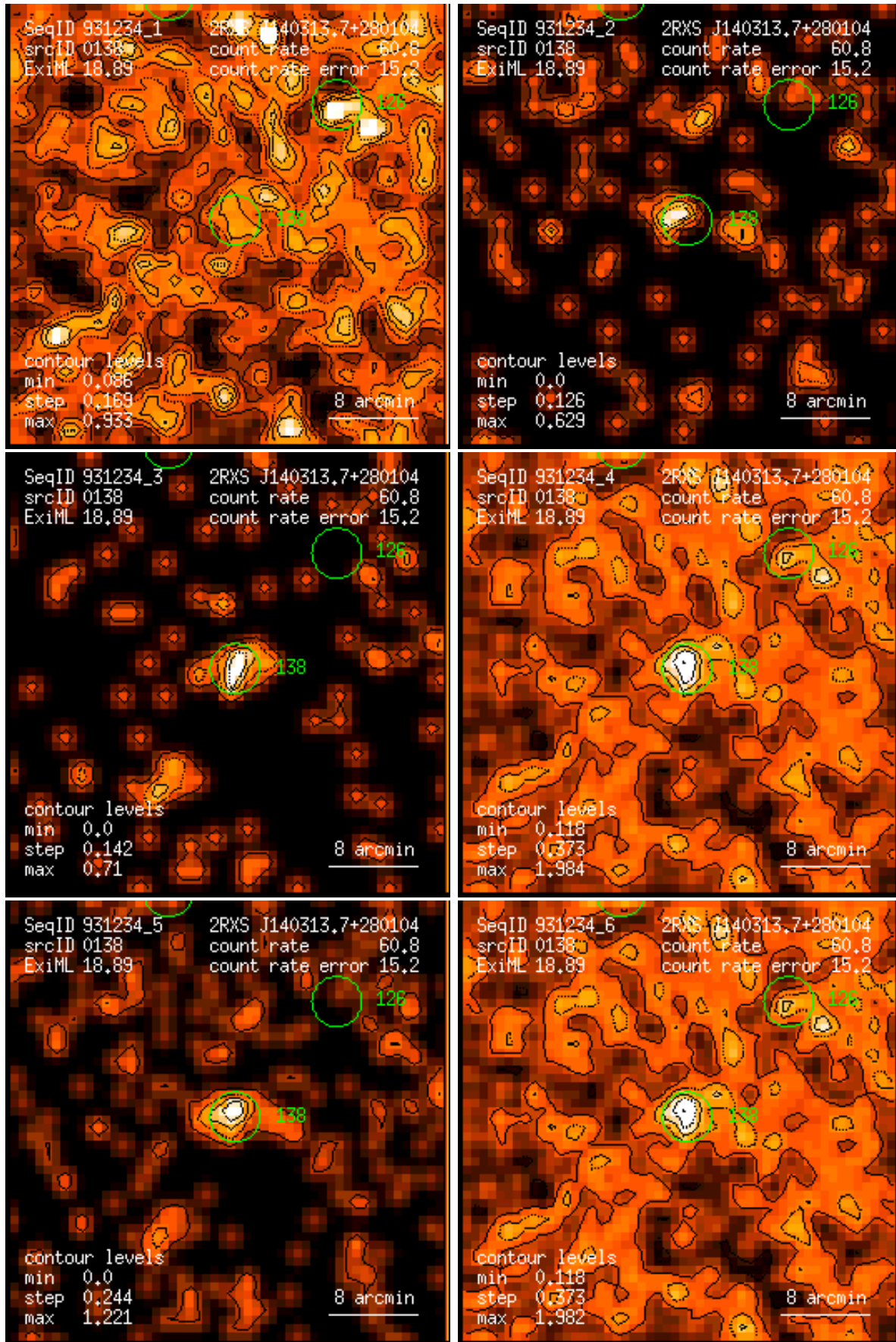
Figure 138: RASS 931234: detection 0138: band rate images, Gaussian filter: (1) PSPC channels 11 – 41, (2) 52 – 90, (3) 91 – 201, (4) 11 – 235, (5) 52 – 201, (6) 11 – 201. Broad band rates in counts/ks. Band rate contour levels in counts/ks/arcmin 2 .
