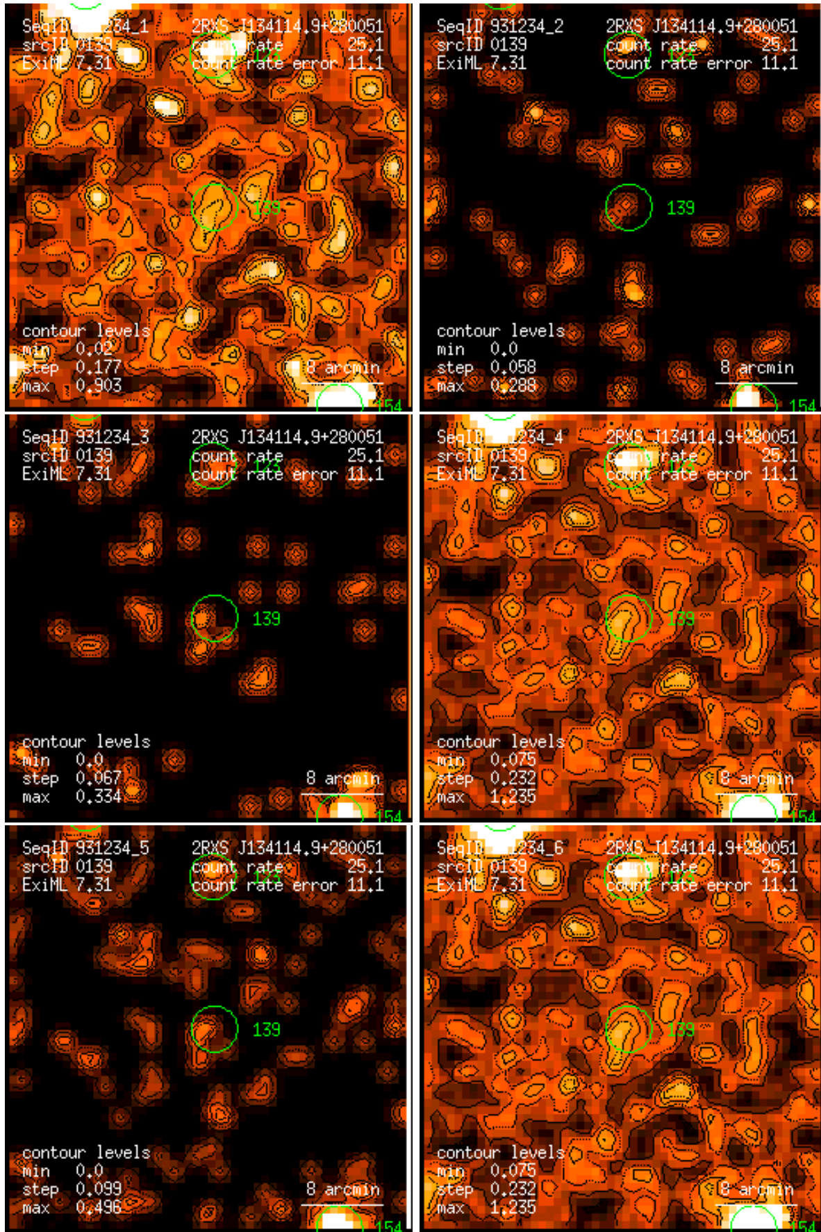
Figure 139: RASS 931234: detection 0139: band rate images, Gaussian filter: (1) PSPC channels 11 – 41, (2) 52 – 90, (3) 91 – 201, (4) 11 – 235, (5) 52 – 201, (6) 11 – 201. Broad band rates in counts/ks. Band rate contour levels in counts/ks/arcmin 2 .
