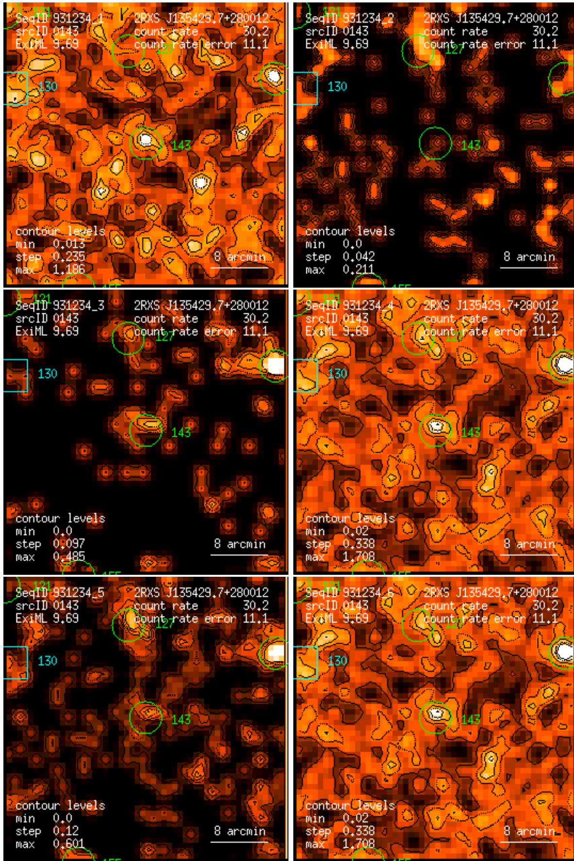
Figure 143: RASS 931234: detection 0143: band rate images, Gaussian filter: (1) PSPC channels 11 – 41, (2) 52 – 90, (3) 91 – 201, (4) 11 – 235, (5) 52 – 201, (6) 11 – 201. Broad band rates in counts/ks. Band rate contour levels in counts/ks/arcmin 2 .
