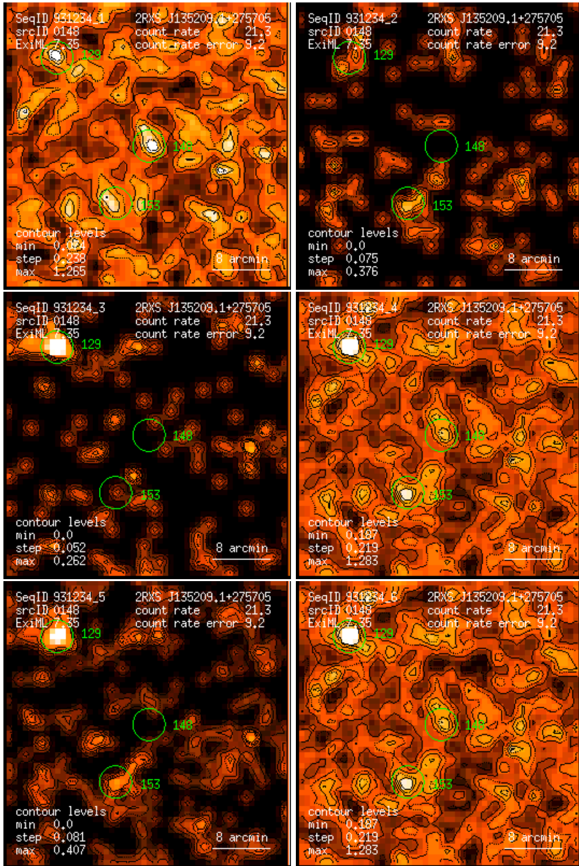
Figure 148: RASS 931234: detection 0148: band rate images, Gaussian filter: (1) PSPC channels 11 – 41, (2) 52 – 90, (3) 91 – 201, (4) 11 – 235, (5) 52 – 201, (6) 11 – 201. Broad band rates in counts/ks. Band rate contour levels in counts/ks/arcmin 2 .
