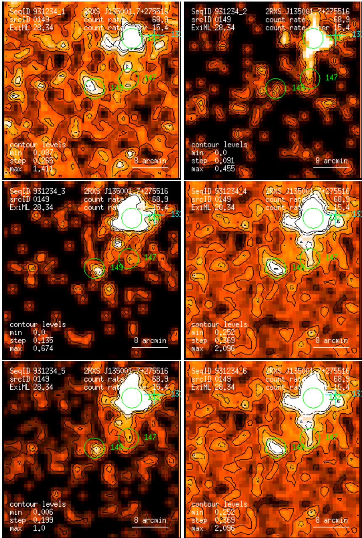
Figure 149: RASS 931234: detection 0149: band rate images, Gaussian filter: (1) PSPC channels 11 – 41, (2) 52 – 90, (3) 91 – 201, (4) 11 – 235, (5) 52 – 201, (6) 11 – 201. Broad band rates in counts/ks. Band rate contour levels in counts/ks/arcmin 2 .
