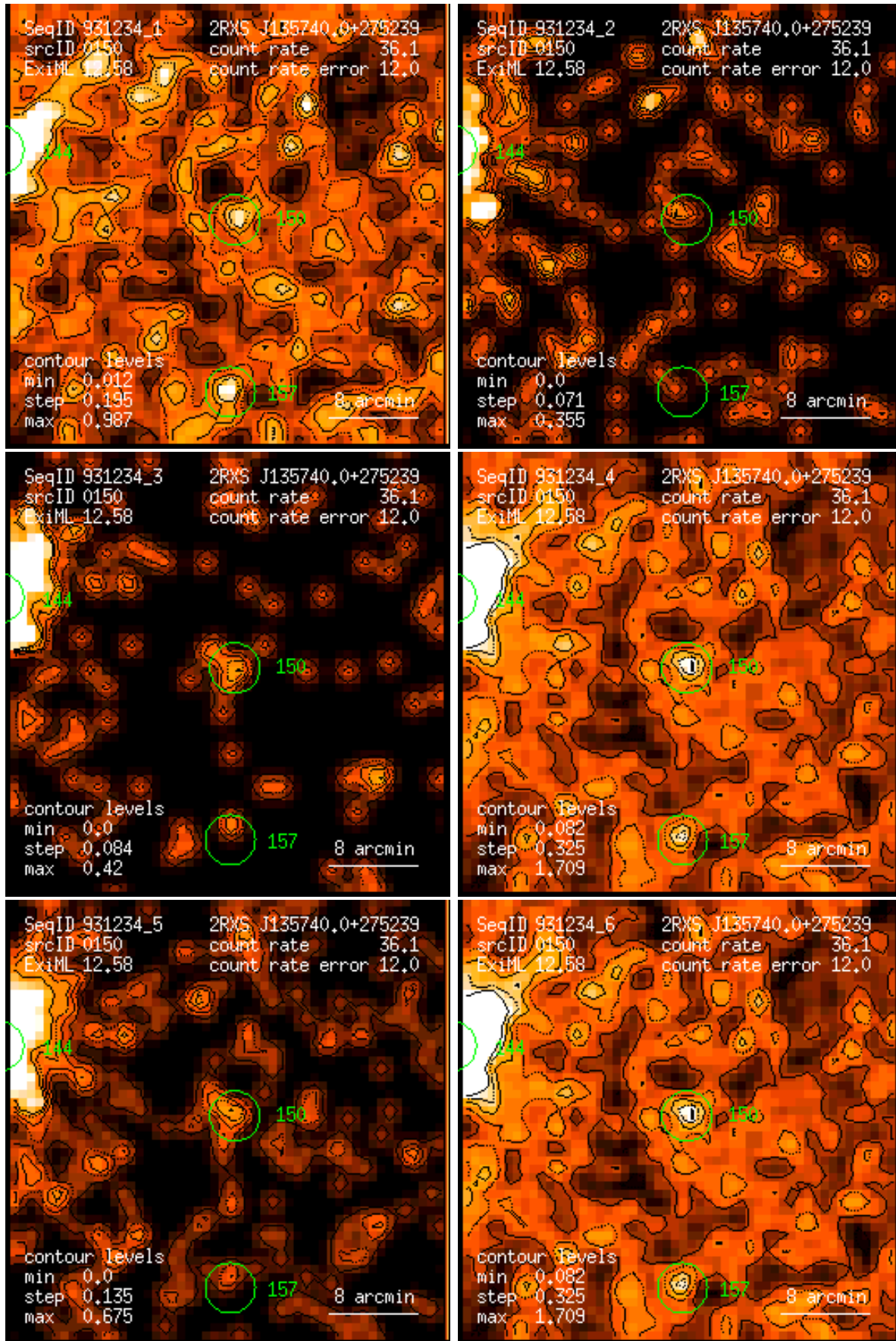
Figure 150: RASS 931234: detection 0150: band rate images, Gaussian filter: (1) PSPC channels 11 – 41, (2) 52 – 90, (3) 91 – 201, (4) 11 – 235, (5) 52 – 201, (6) 11 – 201. Broad band rates in counts/ks. Band rate contour levels in counts/ks/arcmin 2 .
