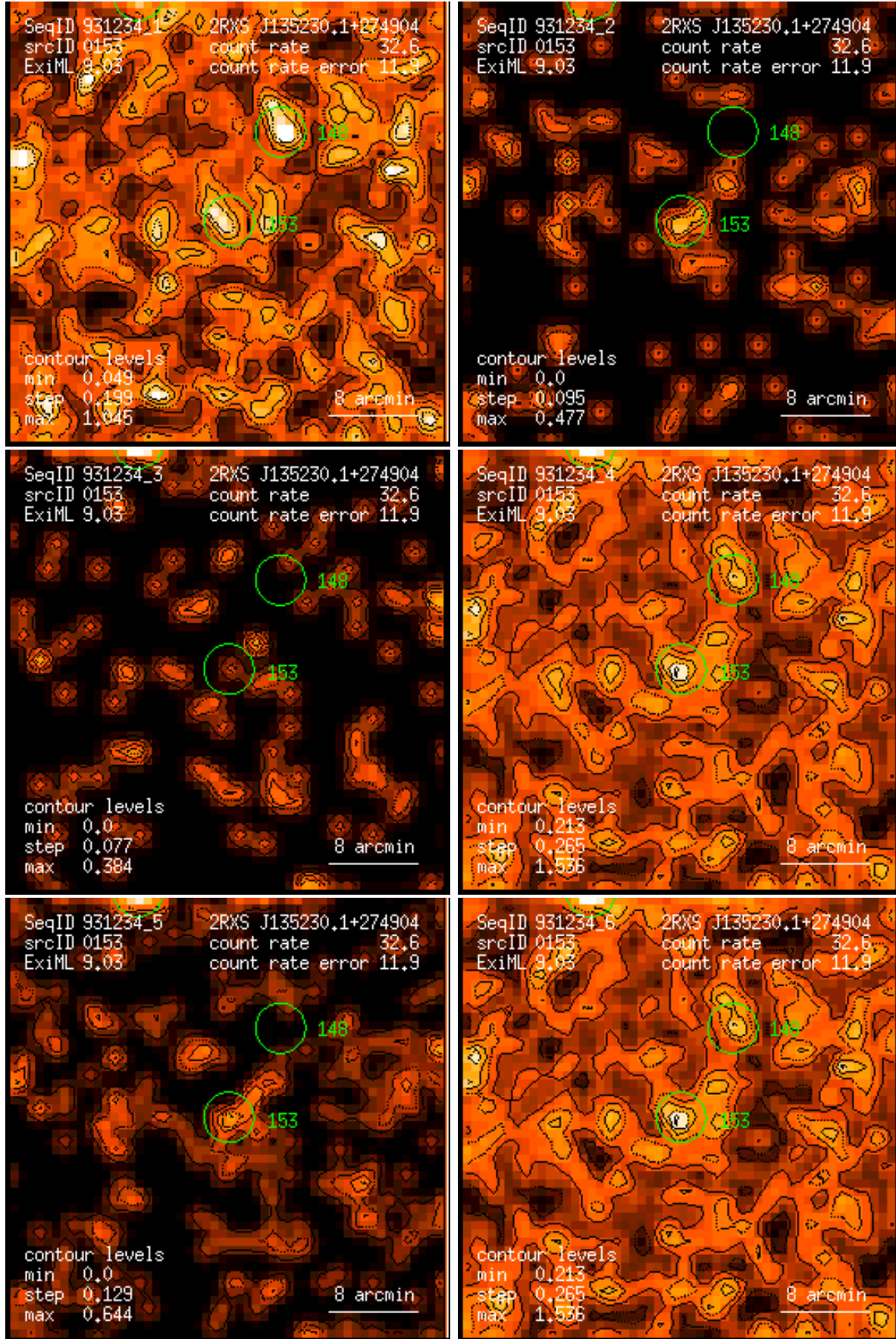
Figure 153: RASS 931234: detection 0153: band rate images, Gaussian filter: (1) PSPC channels 11 – 41, (2) 52 – 90, (3) 91 – 201, (4) 11 – 235, (5) 52 – 201, (6) 11 – 201. Broad band rates in counts/ks. Band rate contour levels in counts/ks/arcmin 2 .
