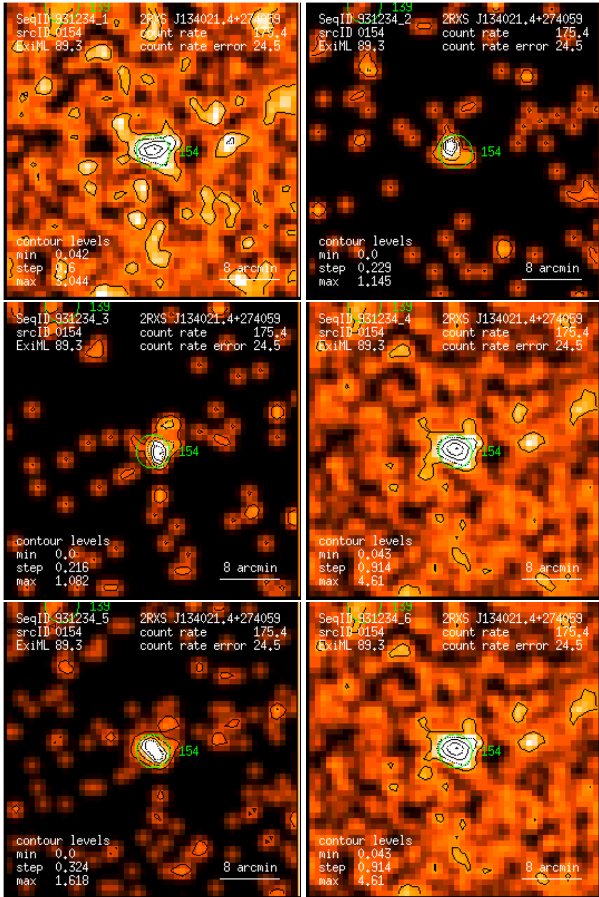
Figure 154: RASS 931234: detection 0154: band rate images, Gaussian filter: (1) PSPC channels 11 – 41, (2) 52 – 90, (3) 91 – 201, (4) 11 – 235, (5) 52 – 201, (6) 11 – 201. Broad band rates in counts/ks. Band rate contour levels in counts/ks/arcmin 2 .
