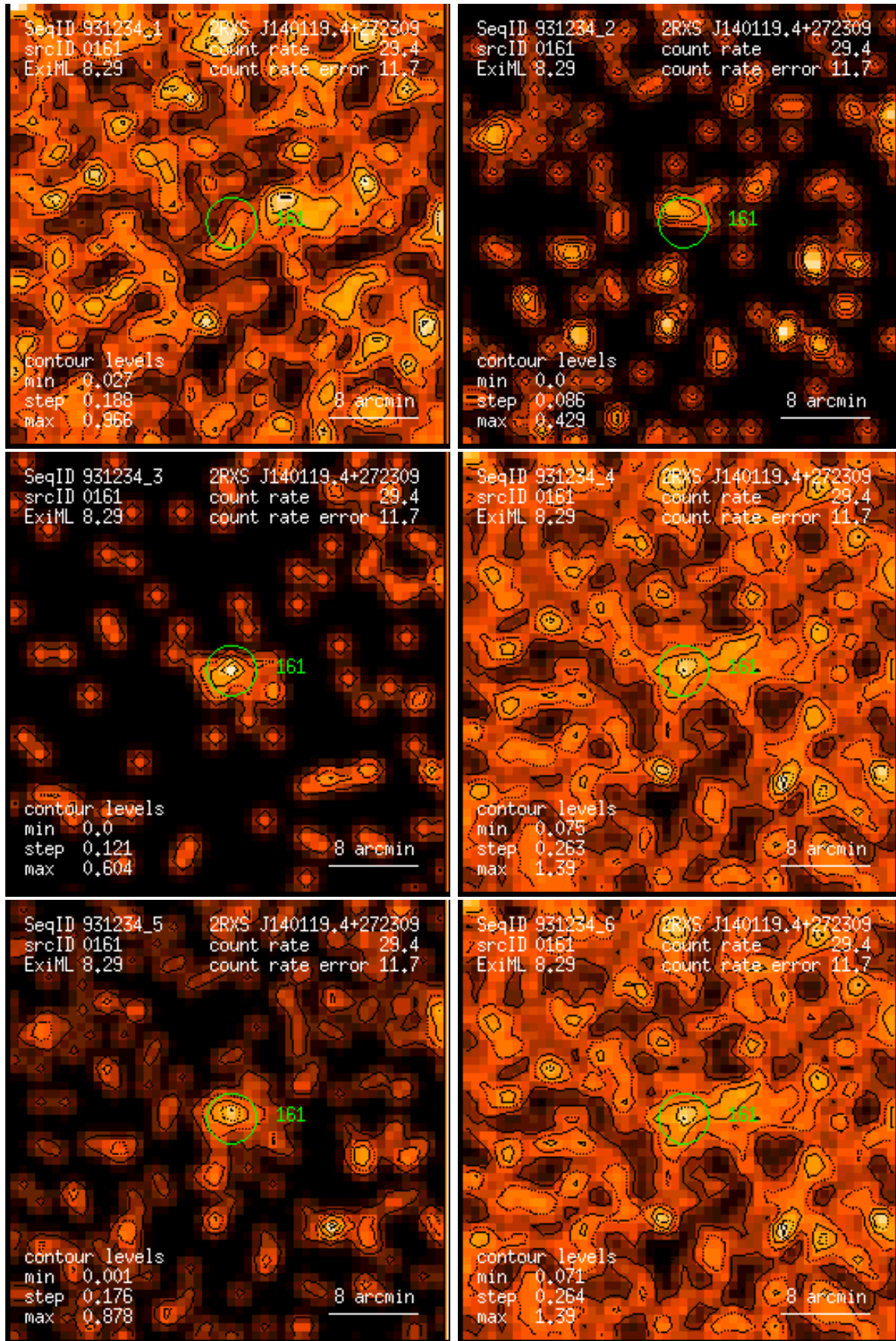
Figure 161: RASS 931234: detection 0161: band rate images, Gaussian filter: (1) PSPC channels 11 – 41, (2) 52 – 90, (3) 91 – 201, (4) 11 – 235, (5) 52 – 201, (6) 11 – 201. Broad band rates in counts/ks. Band rate contour levels in counts/ks/arcmin 2 .
