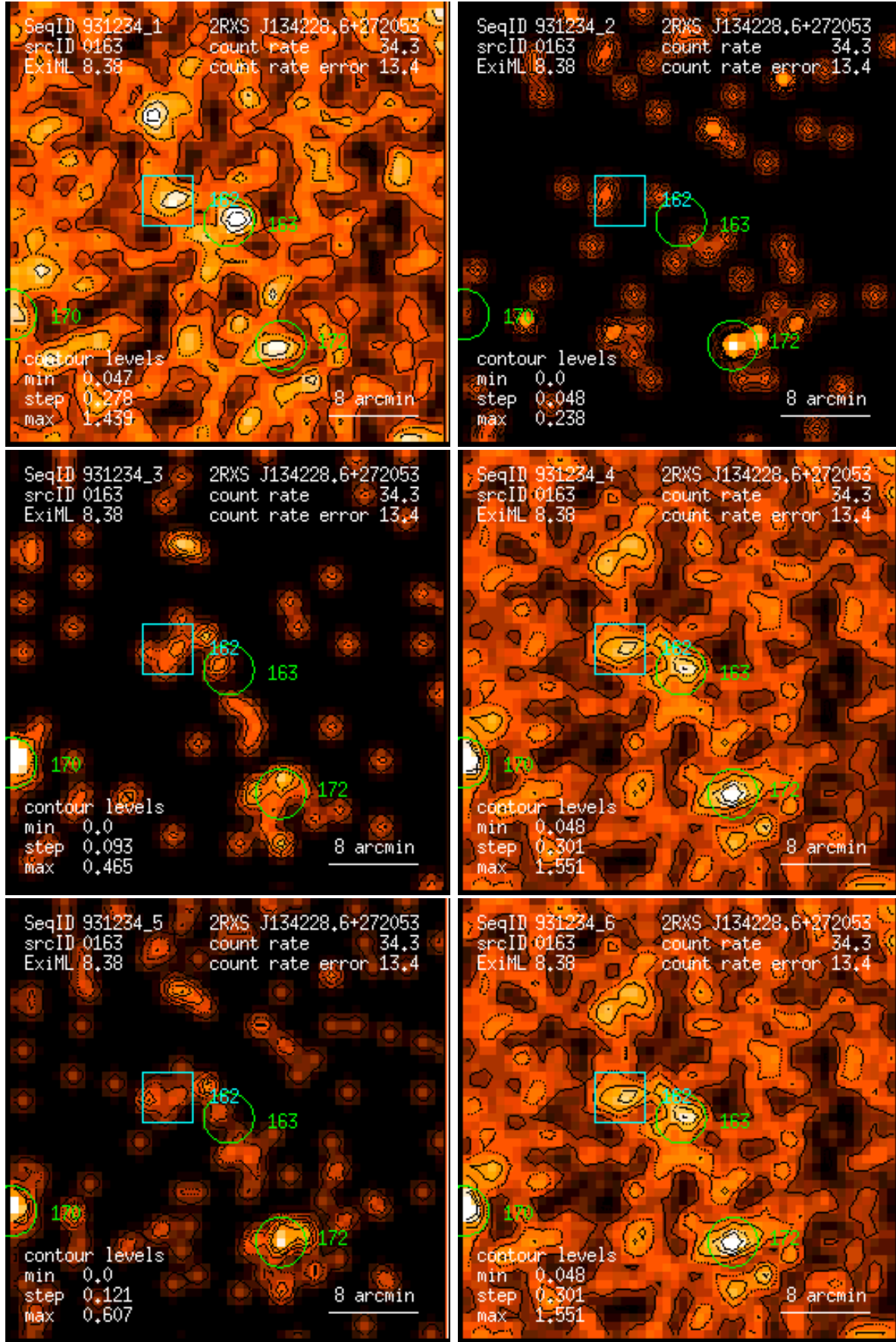
Figure 163: RASS 931234: detection 0163: band rate images, Gaussian filter: (1) PSPC channels 11 – 41, (2) 52 – 90, (3) 91 – 201, (4) 11 – 235, (5) 52 – 201, (6) 11 – 201. Broad band rates in counts/ks. Band rate contour levels in counts/ks/arcmin 2 .
