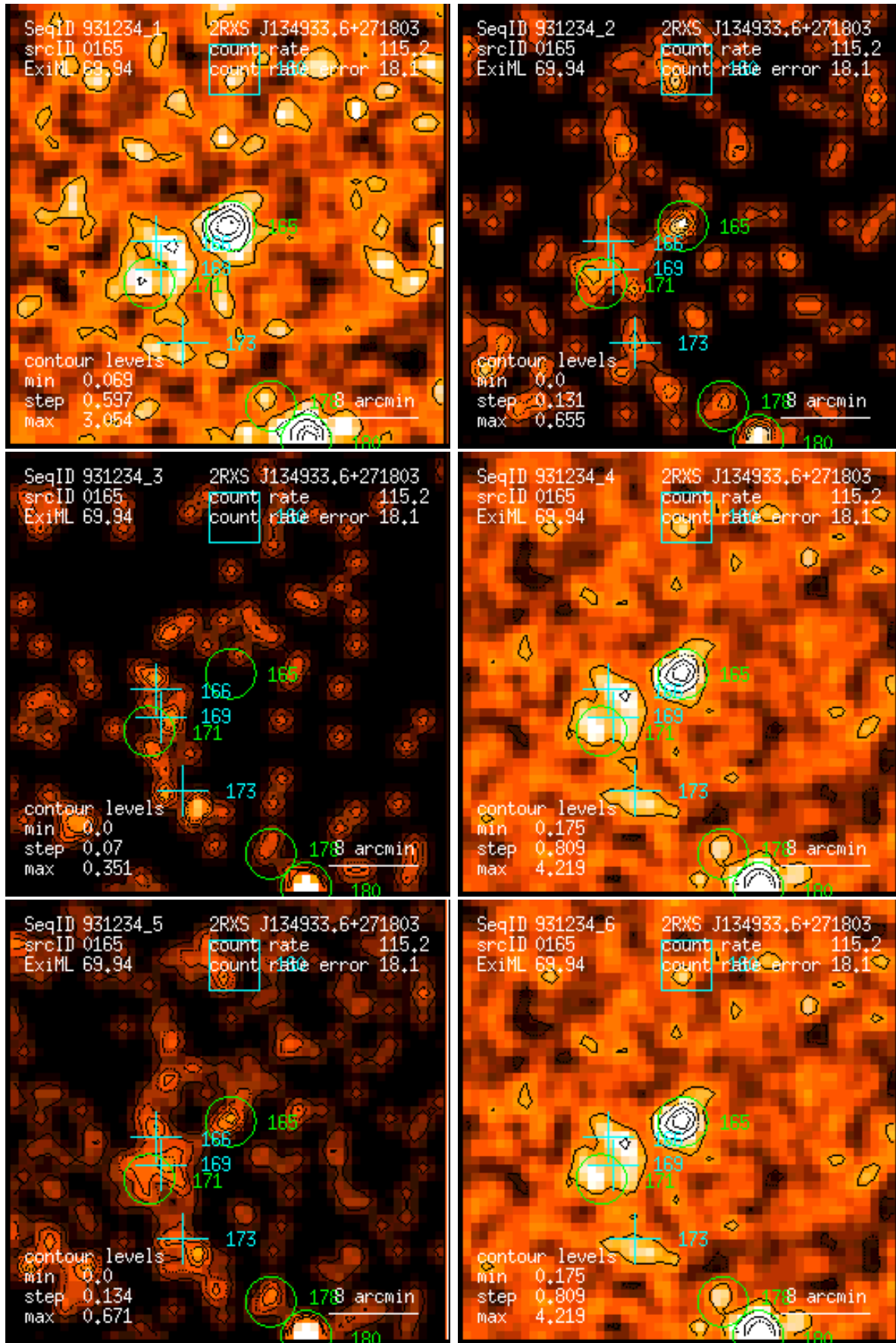
Figure 165: RASS 931234: detection 0165: band rate images, Gaussian filter: (1) PSPC channels 11 – 41, (2) 52 – 90, (3) 91 – 201, (4) 11 – 235, (5) 52 – 201, (6) 11 – 201. Broad band rates in counts/ks. Band rate contour levels in counts/ks/arcmin 2 .
