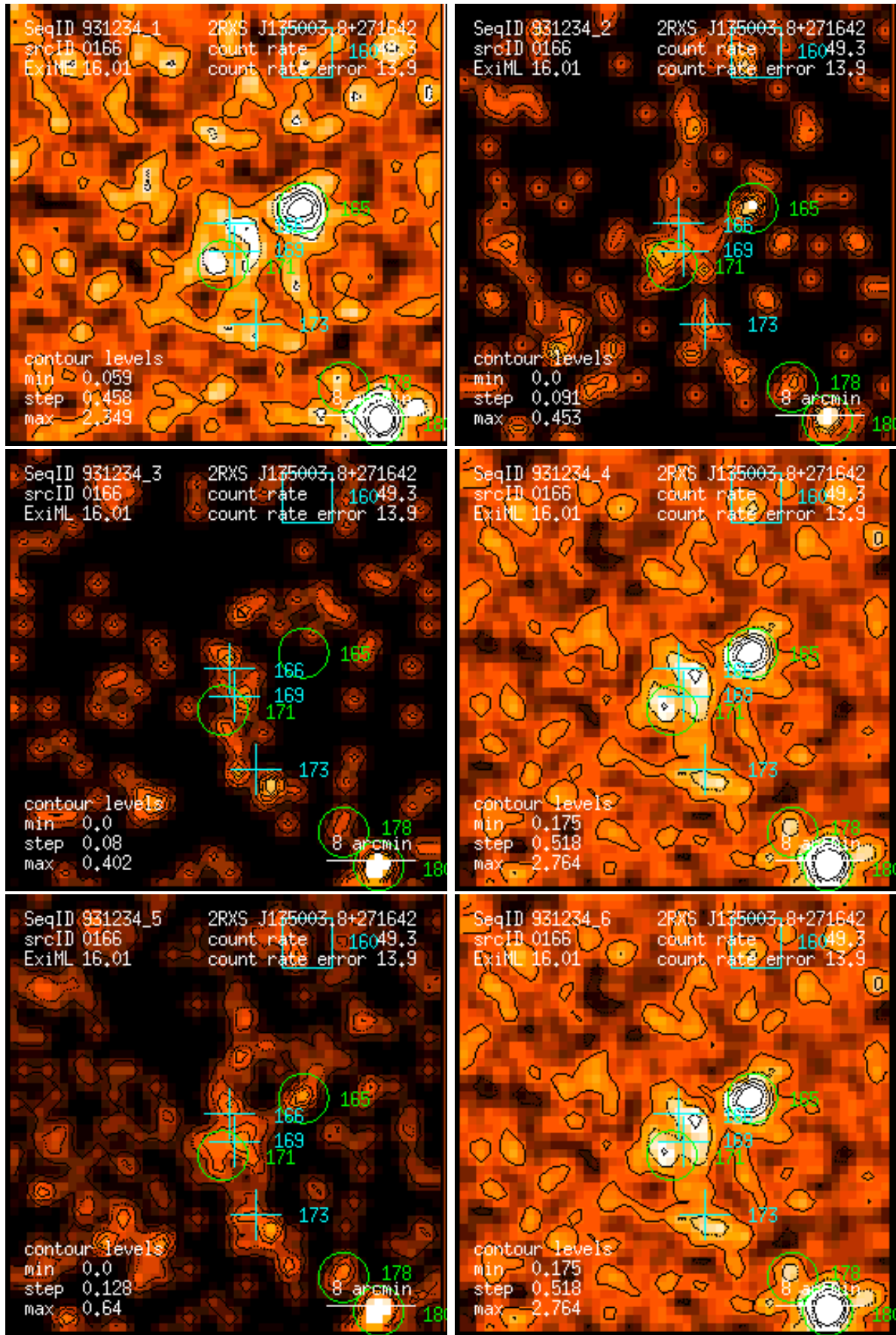
Figure 166: RASS 931234: detection 0166: band rate images, Gaussian filter: (1) PSPC channels 11 – 41, (2) 52 – 90, (3) 91 – 201, (4) 11 – 235, (5) 52 – 201, (6) 11 – 201. Broad band rates in counts/ks. Band rate contour levels in counts/ks/arcmin 2 .
