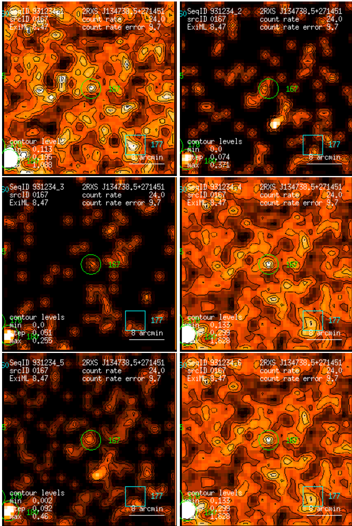
Figure 167: RASS 931234: detection 0167: band rate images, Gaussian filter: (1) PSPC channels 11 – 41, (2) 52 – 90, (3) 91 – 201, (4) 11 – 235, (5) 52 – 201, (6) 11 – 201. Broad band rates in counts/ks. Band rate contour levels in counts/ks/arcmin 2 .
