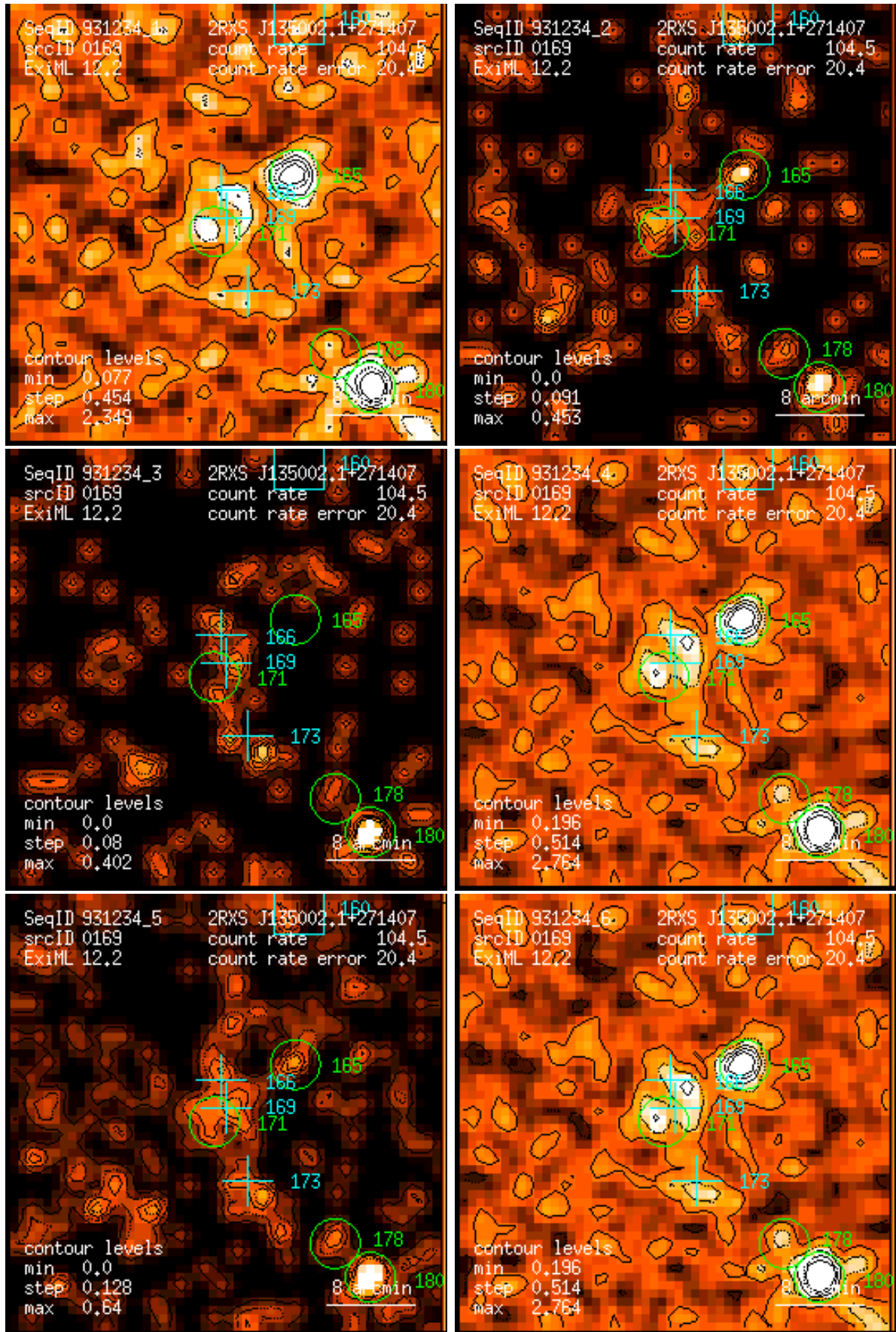
Figure 169: RASS 931234: detection 0169: band rate images, Gaussian filter: (1) PSPC channels 11 – 41, (2) 52 – 90, (3) 91 – 201, (4) 11 – 235, (5) 52 – 201, (6) 11 – 201. Broad band rates in counts/ks. Band rate contour levels in counts/ks/arcmin 2 .
