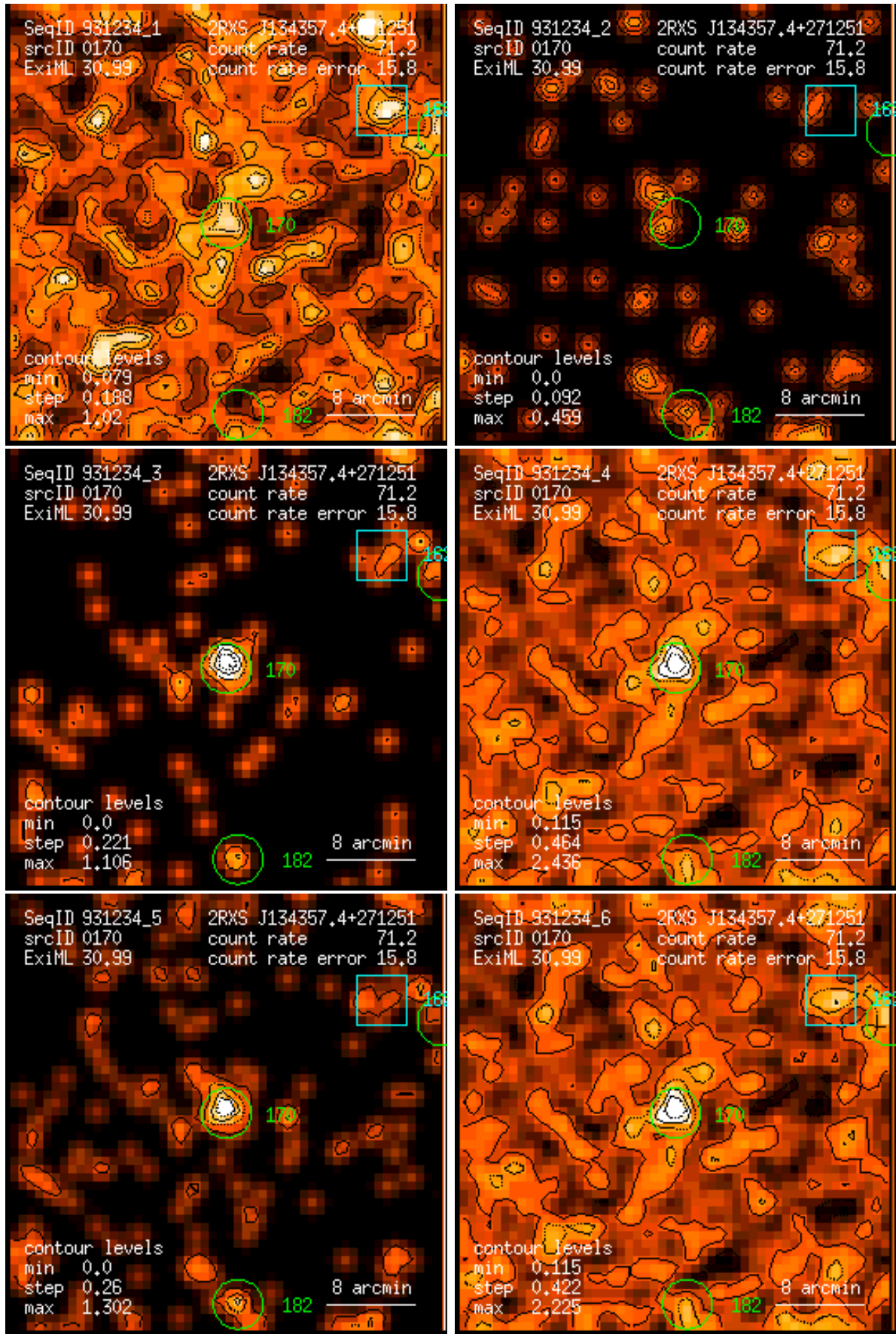
Figure 170: RASS 931234: detection 0170: band rate images, Gaussian filter: (1) PSPC channels 11 – 41, (2) 52 – 90, (3) 91 – 201, (4) 11 – 235, (5) 52 – 201, (6) 11 – 201. Broad band rates in counts/ks. Band rate contour levels in counts/ks/arcmin 2 .
