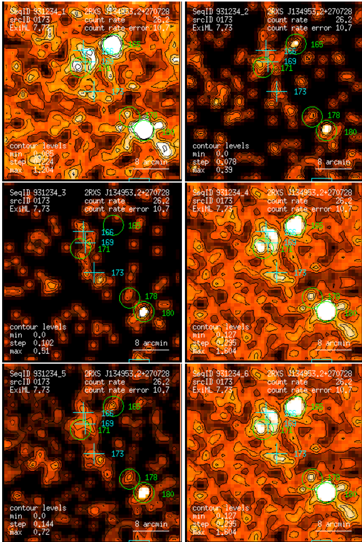
Figure 173: RASS 931234: detection 0173: band rate images, Gaussian filter: (1) PSPC channels 11 – 41, (2) 52 – 90, (3) 91 – 201, (4) 11 – 235, (5) 52 – 201, (6) 11 – 201. Broad band rates in counts/ks. Band rate contour levels in counts/ks/arcmin 2 .
