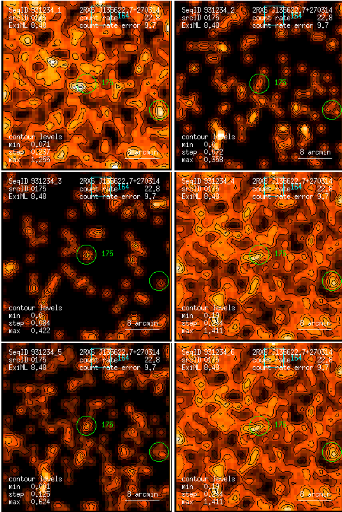
Figure 175: RASS 931234: detection 0175: band rate images, Gaussian filter: (1) PSPC channels 11 – 41, (2) 52 – 90, (3) 91 – 201, (4) 11 – 235, (5) 52 – 201, (6) 11 – 201. Broad band rates in counts/ks. Band rate contour levels in counts/ks/arcmin 2 .
