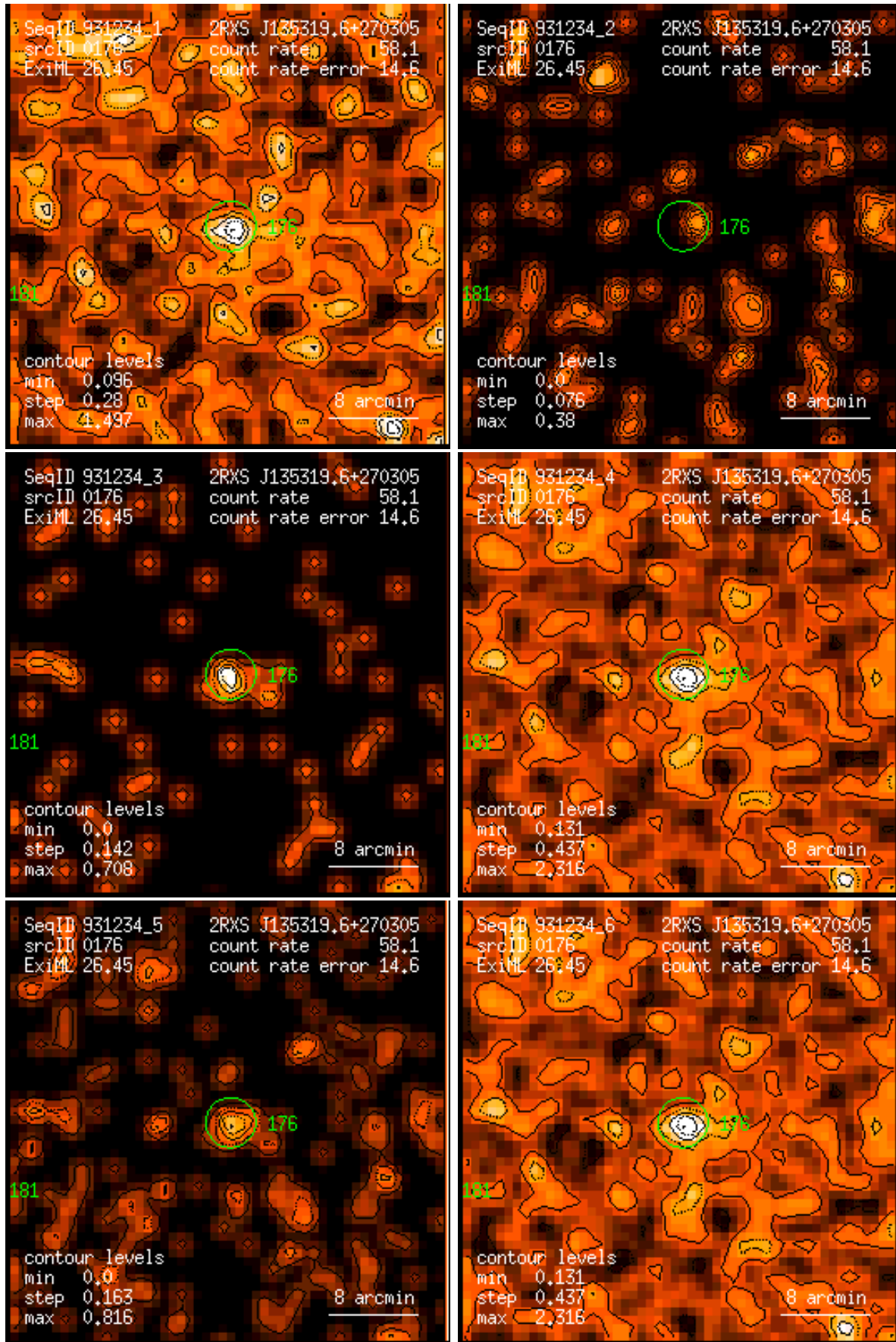
Figure 176: RASS 931234: detection 0176: band rate images, Gaussian filter: (1) PSPC channels 11 – 41, (2) 52 – 90, (3) 91 – 201, (4) 11 – 235, (5) 52 – 201, (6) 11 – 201. Broad band rates in counts/ks. Band rate contour levels in counts/ks/arcmin 2 .
