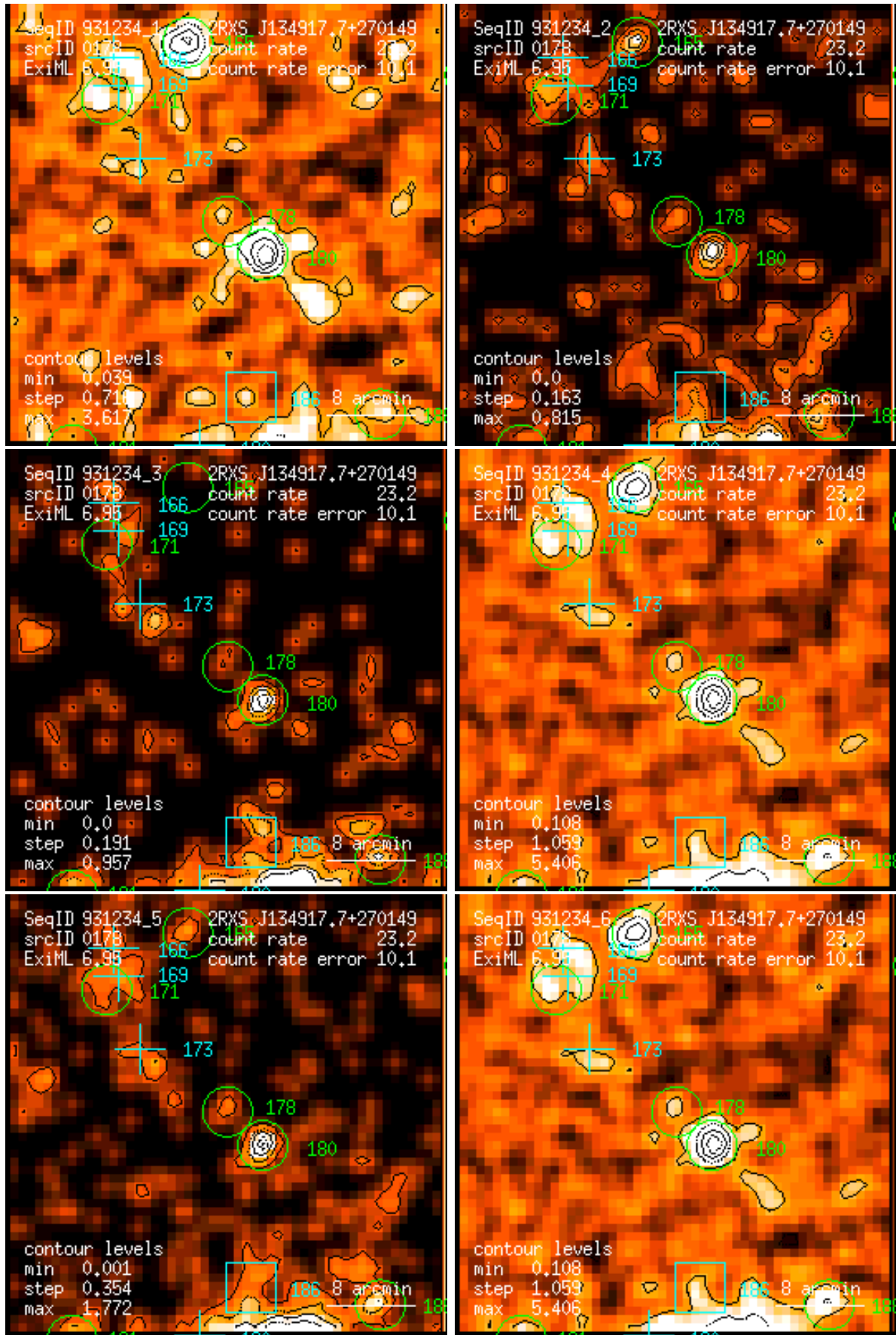
Figure 178: RASS 931234: detection 0178: band rate images, Gaussian filter: (1) PSPC channels 11 – 41, (2) 52 – 90, (3) 91 – 201, (4) 11 – 235, (5) 52 – 201, (6) 11 – 201. Broad band rates in counts/ks. Band rate contour levels in counts/ks/arcmin 2 .
