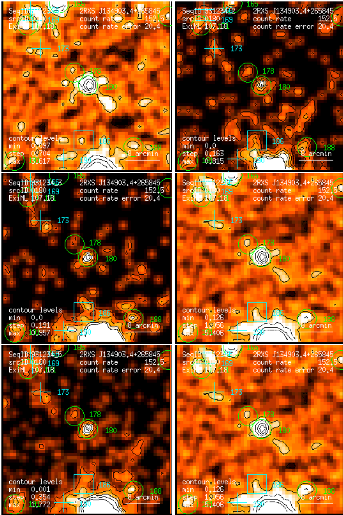
Figure 180: RASS 931234: detection 0180: band rate images, Gaussian filter: (1) PSPC channels 11 – 41, (2) 52 – 90, (3) 91 – 201, (4) 11 – 235, (5) 52 – 201, (6) 11 – 201. Broad band rates in counts/ks. Band rate contour levels in counts/ks/arcmin 2 .
