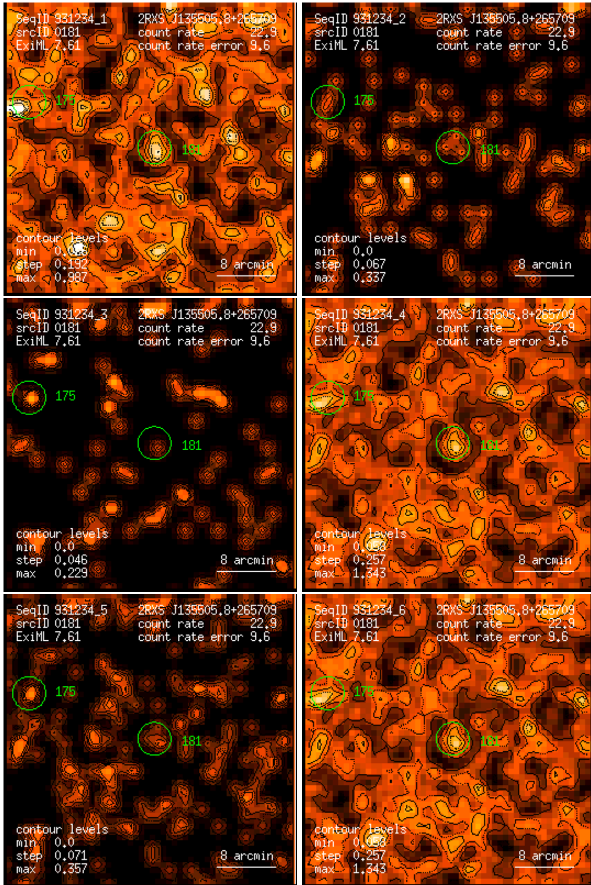
Figure 181: RASS 931234: detection 0181: band rate images, Gaussian filter: (1) PSPC channels 11 – 41, (2) 52 – 90, (3) 91 – 201, (4) 11 – 235, (5) 52 – 201, (6) 11 – 201. Broad band rates in counts/ks. Band rate contour levels in counts/ks/arcmin 2 .
