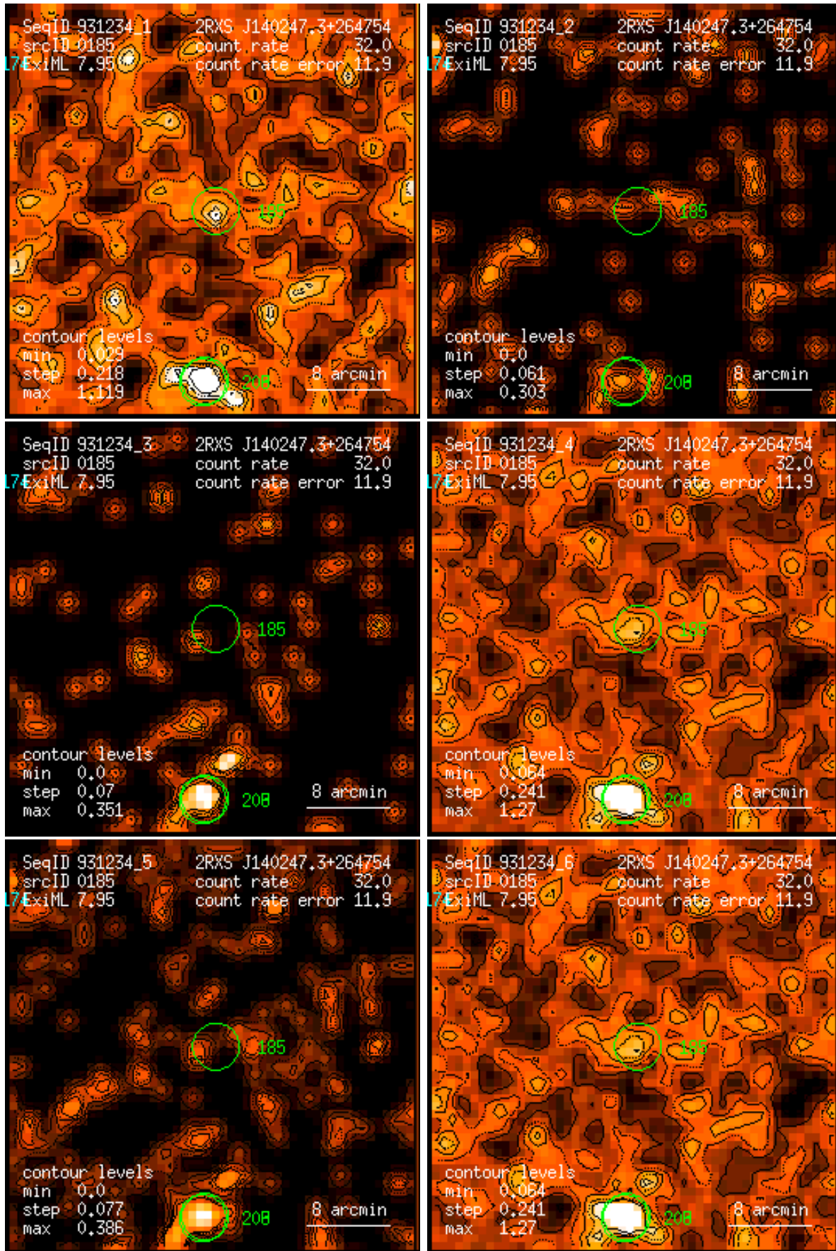
Figure 185: RASS 931234: detection 0185: band rate images, Gaussian filter: (1) PSPC channels 11 – 41, (2) 52 – 90, (3) 91 – 201, (4) 11 – 235, (5) 52 – 201, (6) 11 – 201. Broad band rates in counts/ks. Band rate contour levels in counts/ks/arcmin 2 .
