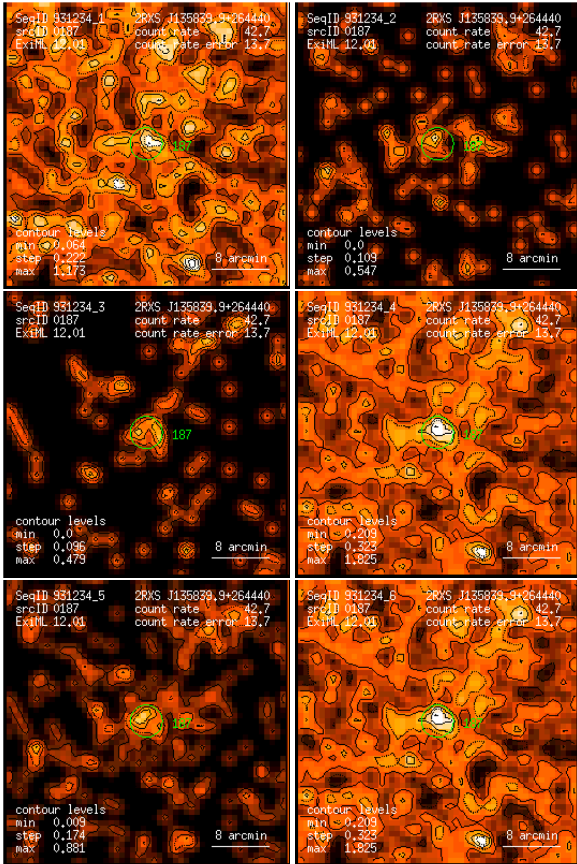
Figure 187: RASS 931234: detection 0187: band rate images, Gaussian filter: (1) PSPC channels 11 – 41, (2) 52 – 90, (3) 91 – 201, (4) 11 – 235, (5) 52 – 201, (6) 11 – 201. Broad band rates in counts/ks. Band rate contour levels in counts/ks/arcmin 2 .
