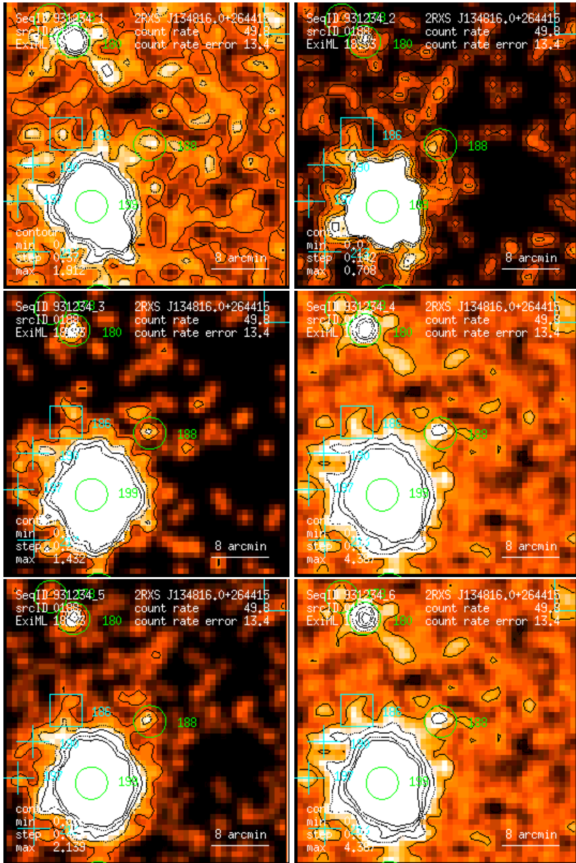
Figure 188: RASS 931234: detection 0188: band rate images, Gaussian filter: (1) PSPC channels 11 – 41, (2) 52 – 90, (3) 91 – 201, (4) 11 – 235, (5) 52 – 201, (6) 11 – 201. Broad band rates in counts/ks. Band rate contour levels in counts/ks/arcmin 2 .
