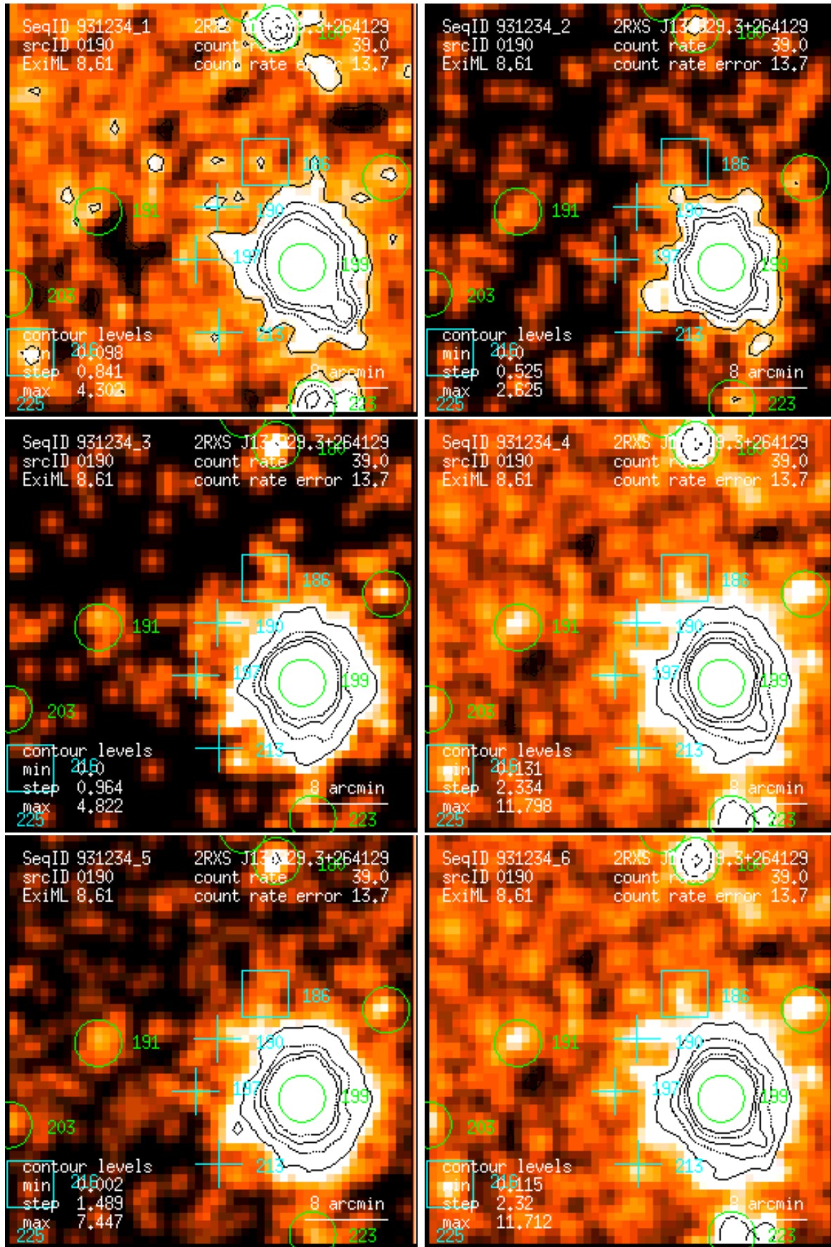
Figure 190: RASS 931234: detection 0190: band rate images, Gaussian filter: (1) PSPC channels 11 – 41, (2) 52 – 90, (3) 91 – 201, (4) 11 – 235, (5) 52 – 201, (6) 11 – 201. Broad band rates in counts/ks. Band rate contour levels in counts/ks/arcmin 2 .
