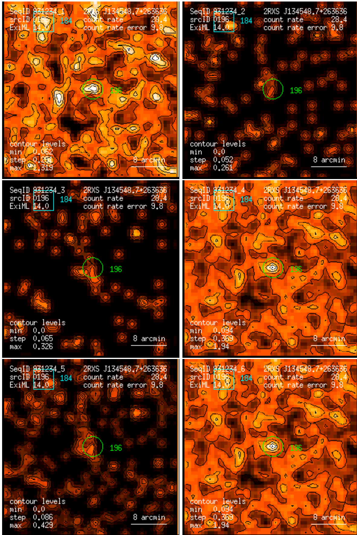
Figure 196: RASS 931234: detection 0196: band rate images, Gaussian filter: (1) PSPC channels 11 – 41, (2) 52 – 90, (3) 91 – 201, (4) 11 – 235, (5) 52 – 201, (6) 11 – 201. Broad band rates in counts/ks. Band rate contour levels in counts/ks/arcmin 2 .
