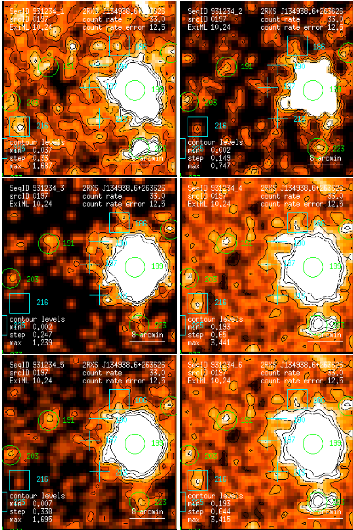
Figure 197: RASS 931234: detection 0197: band rate images, Gaussian filter: (1) PSPC channels 11 – 41, (2) 52 – 90, (3) 91 – 201, (4) 11 – 235, (5) 52 – 201, (6) 11 – 201. Broad band rates in counts/ks. Band rate contour levels in counts/ks/arcmin 2 .
