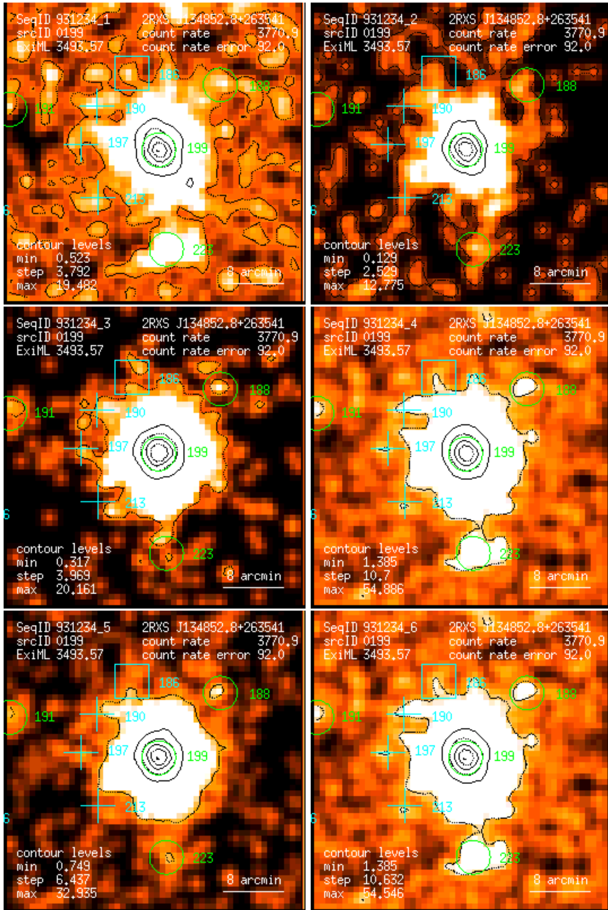
Figure 199: RASS 931234: detection 0199: band rate images, Gaussian filter: (1) PSPC channels 11 – 41, (2) 52 – 90, (3) 91 – 201, (4) 11 – 235, (5) 52 – 201, (6) 11 – 201. Broad band rates in counts/ks. Band rate contour levels in counts/ks/arcmin 2 .
